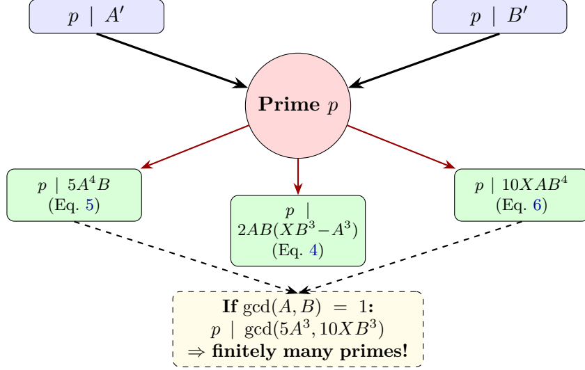
Figure 4: The ABC Prime Isolation Funnel. Any prime p invading both A' and B' is forced through three independent modular constraints, each proven by Lean 4. When \gcd(A, B) = 1 , the set of admissible primes collapses to a finite, bounded collection.
