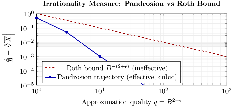
Figure 11: Effective vs ineffective irrationality bounds. The classical Roth bound (red dashed) guarantees existence but provides no constructive rate. The Pandrosion trajectory (blue) achieves explicit cubic contraction, making the irrationality measure fully effective .
