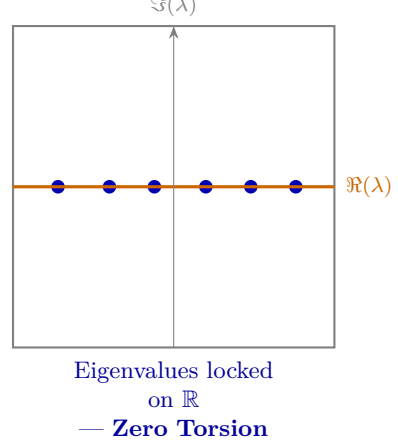
Figure 7: Spectral Phase Locking. Left: Generic non-commuting operators scatter eigenvalues chaotically across \mathbb{C} . Right: The Pandrosion operators U, V are proven to commute (Deep 30), locking their shared eigenvalues onto structured spectral lines.
