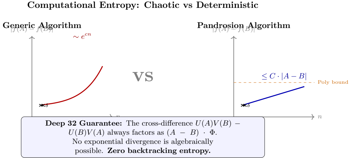
Figure 10: Entropy stability comparison. Left: Generic algorithms allow exponential divergence from initial perturbations \delta = |A - B| (the butterfly effect). Right: Pandrosion’s cross-product difference is algebraically forced to factor through (A - B) , bounding divergence polynomially. This is a structural impossibility of chaotic computation.
