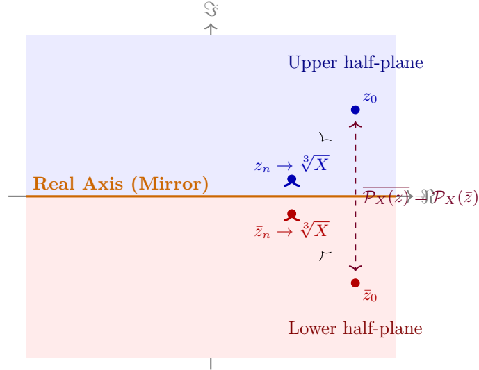
Figure 6: Conjugate symmetry (Deep 29). Every trajectory z_0 \rightarrow z_n in the upper half-plane is mirrored perfectly by \bar{z}_0 \rightarrow \bar{z}_n in the lower half-plane. This topological congruence eliminates asymmetric fractal boundary formation.
