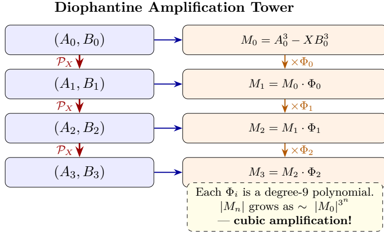
Figure 3: The Diophantine Amplification Tower. Each application of the Pandrosion map multiplies the Pell error M = A^3 - XB^3 by an explicit degree-9 polynomial \Phi , generating an infinite tower of integer solutions to the cubic Thue equation.
