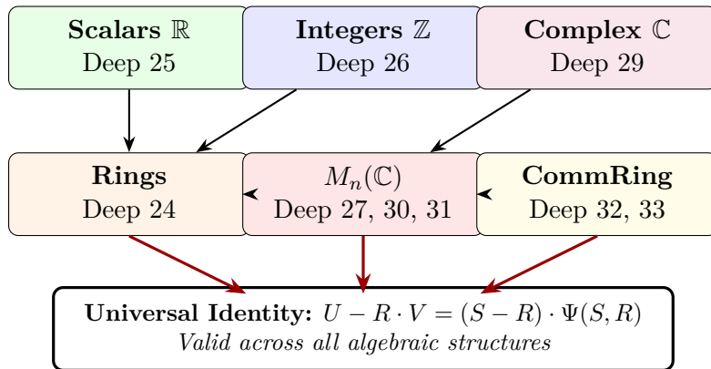
Figure 9: The Algebraic Hierarchy. The Pandrosion error identity propagates across every level of the algebraic tower: from real scalars through integers and complex numbers to arbitrary rings and matrix algebras. Each generalization is certified independently in Lean 4.
