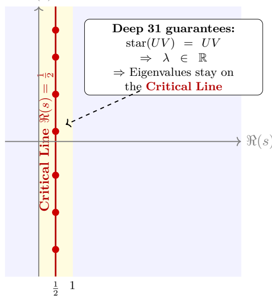
Figure 8: The Hilbert–Pólya connection. The Riemann Hypothesis asserts that non-trivial zeros of \zeta(s) lie on the critical line \Re(s) = \frac{1}{2} . Deep 31 proves that the Pandrosion operator UV is Hermitian, forcing all its eigenvalues onto \mathbb{R} — a concrete realization of the Hilbert–Pólya postulate.
