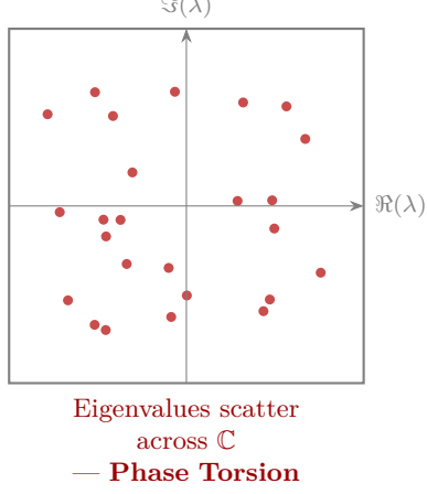
Figure 7: Spectral Phase Locking. Left: Generic non-commuting operators scatter eigenvalues chaotically across \mathbb{C} . Right: The Pandrosion operators U, V are proven to commute (Deep 30), locking their shared eigenvalues onto structured spectral lines.
