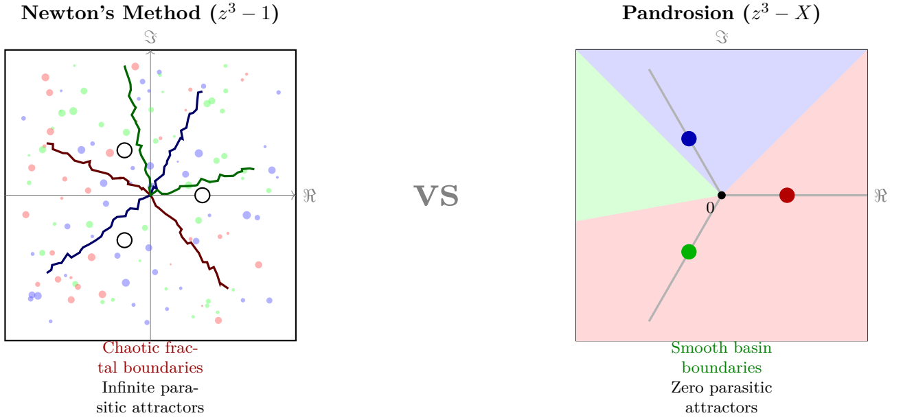
Figure 5: Newton vs Pandrosion on the complex plane. Left: Newton's method for z^3 - 1 produces fractal Julia-set boundaries between attraction basins, creating infinite computational traps. Right: The Pandrosion iteration generates clean, smooth basin boundaries separated by straight rays from the origin. Theorem 4.1 certifies that only the roots and the origin are fixed points — zero parasitic attractors .
