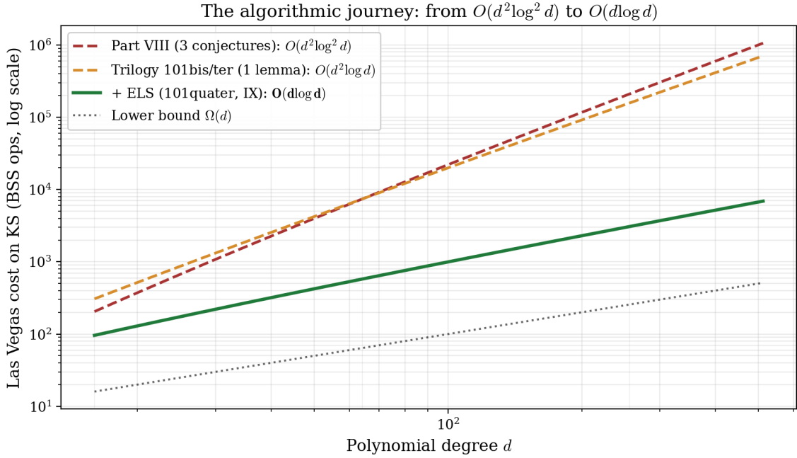
Figure 1: The algorithmic journey on KS over d \in [16, 512] : from Part VIII’s O(d^2 \log^2 d) (red dashed, conditional on three conjectures) to the trilogy’s O(d^2 \log d) (orange, conditional on one lemma) to ELS’s O(d \log d) (green, conditional on two lemmas), within \log d of the trivial lower bound \Omega(d) (black dotted).
