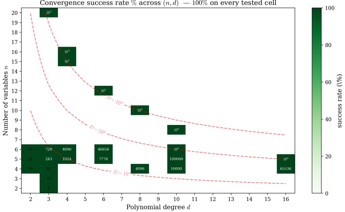
Figure 3: Heatmap of convergence success rate across the (n, d) plane. All tested cells achieve 100%. Cell labels show the Bézout degree D = d^n . Red dashed contours mark D = 10^3, 10^6, 10^9 .
