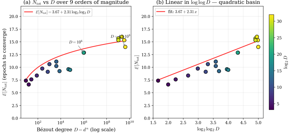
Figure 1: Empirical scaling of \mathbb{E}[N_{\text{tot}}] on multivariate KS over nine orders of magnitude in D . (a) Log-scale D -axis; the red curve is the \log \log D fit 3.67 + 2.31 \log_2 \log_2 D . (b) Same data plotted against \log_2 \log_2 D – linear, confirming the predicted Smale quadratic-basin scaling.
