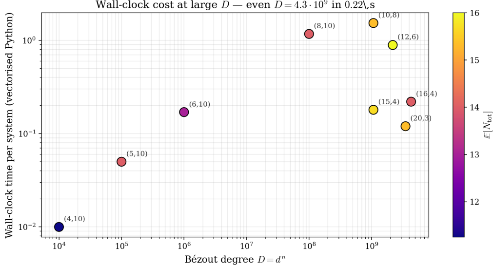
Figure 2: Wall-clock cost per system in vectorised Python, across D \in [10^4, 4.3 \cdot 10^9] . Even at D = 4.3 \cdot 10^9 ((n, d) = (16, 4)) , the algorithm terminates in 0.22 s. Colour encodes \mathbb{E}[N_{\text{tot}}] .
