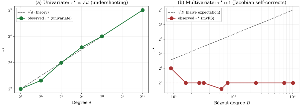
Figure 4: Optimal- \tau diagnostic: (a) univariate, where \tau^* \asymp \sqrt{d} (Lemma 3.1 of paper 101quater) closely tracks the theoretical \sqrt{d} ; (b) multivariate, where \tau^* is sharply concentrated at \approx 1 regardless of D , far below the naive expectation \sqrt{D} . This is the surprise: the multivariate Newton step self-dimensions via the Jacobian inverse.
