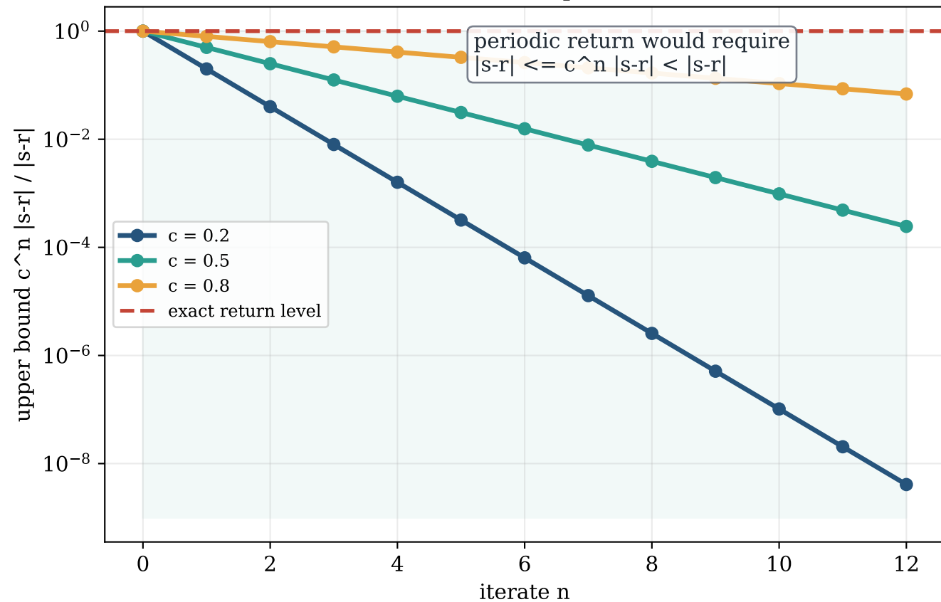
Distance funnel under repeated contraction
