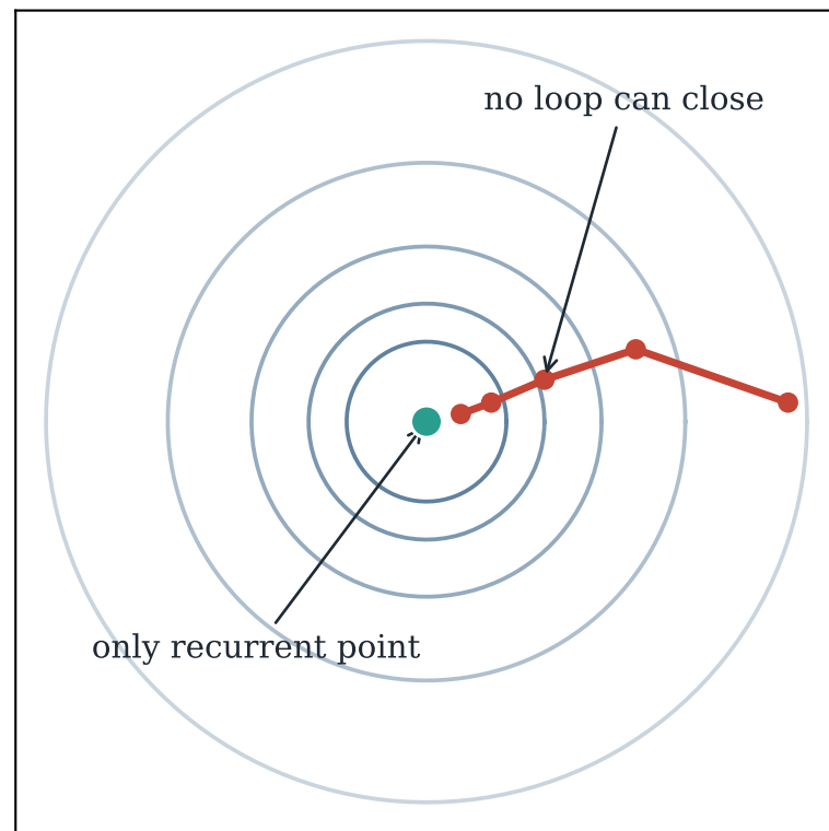
Geometric return obstruction
