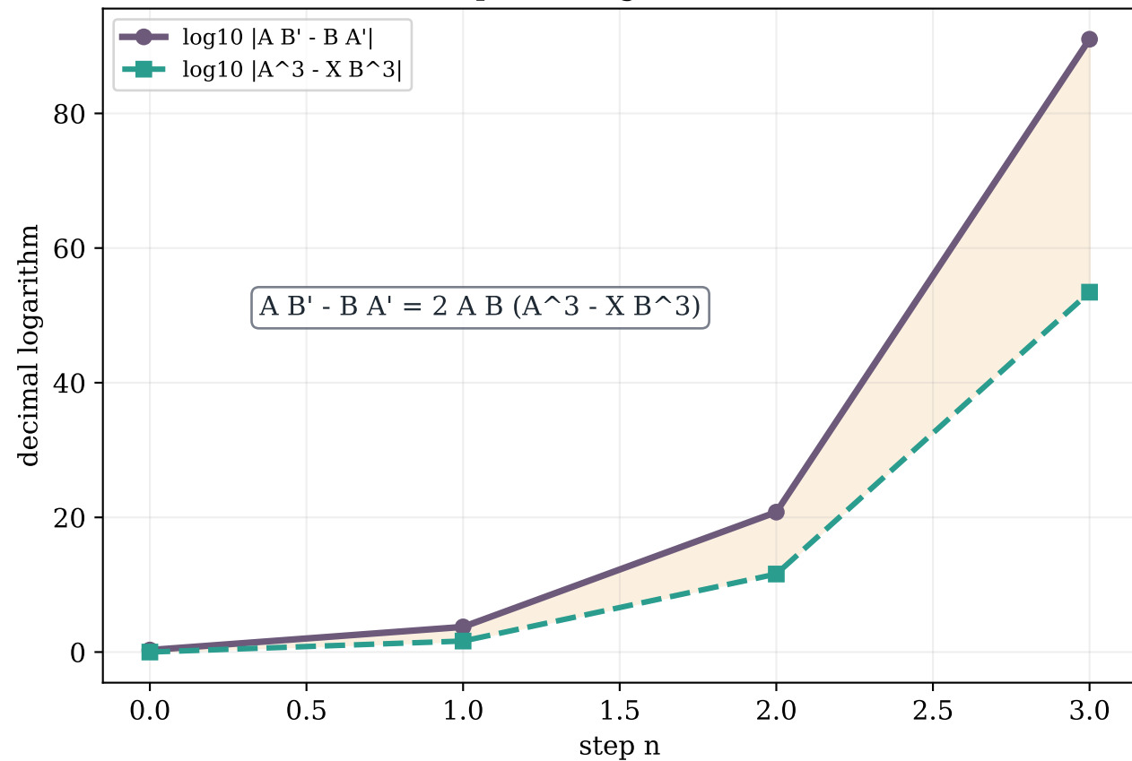
Certified separation grows with the norm
