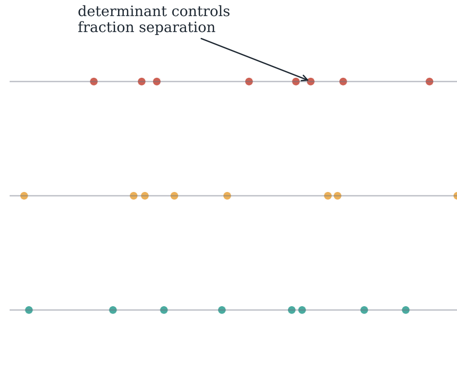
Consecutive approximants separate
