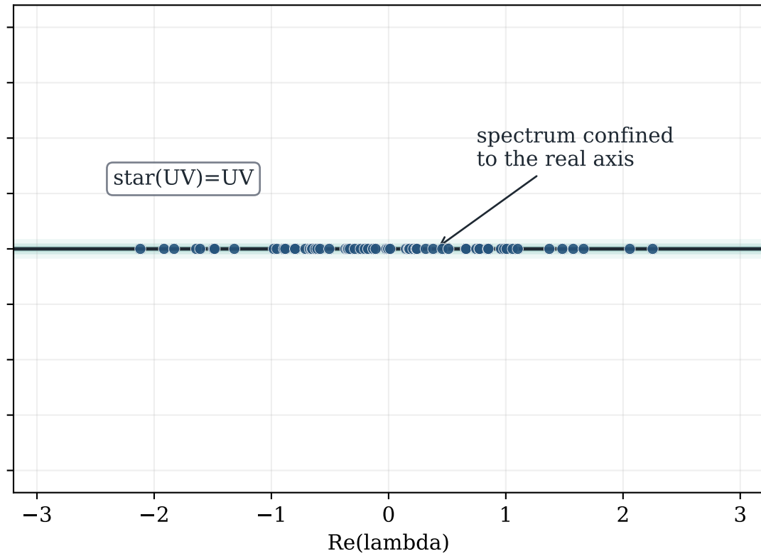
Hermitian Pandrosion product
