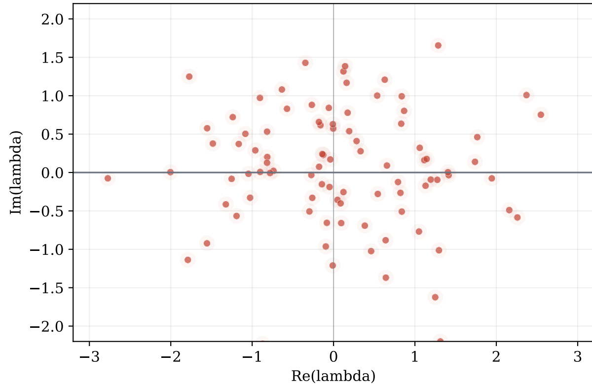
generic complex product
