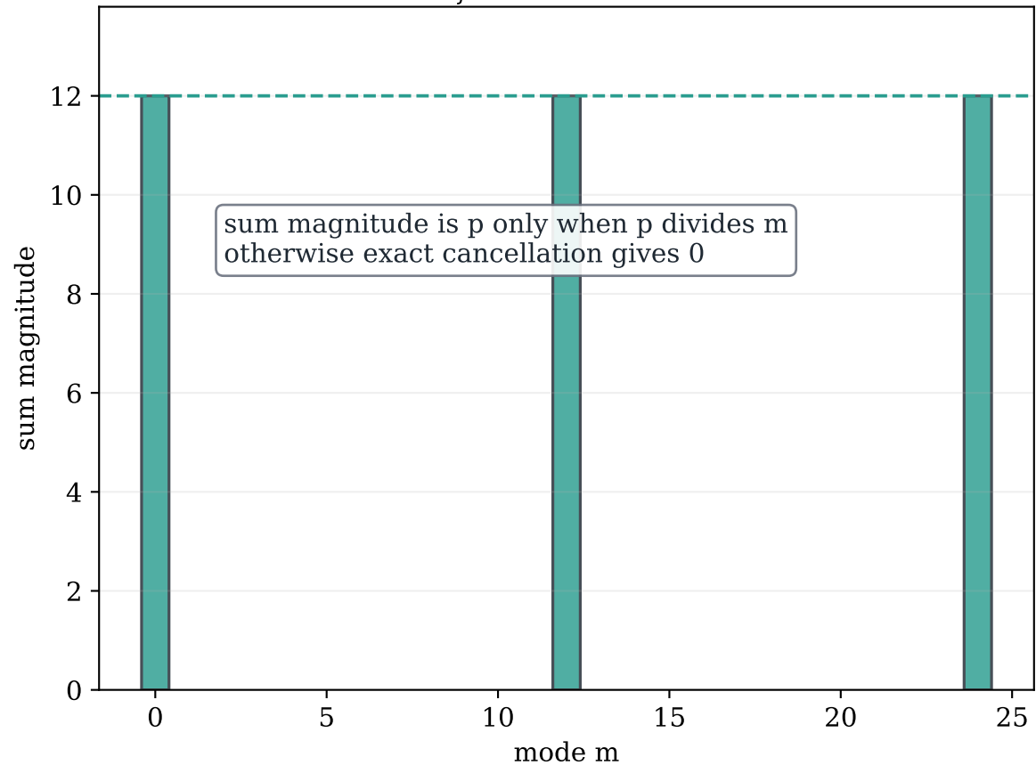
|\sum_j \omega^{jm}| for p=12
