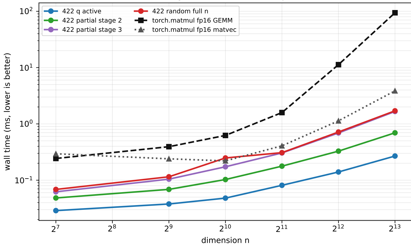
422 runtime against torch.matmul up to n=8192
