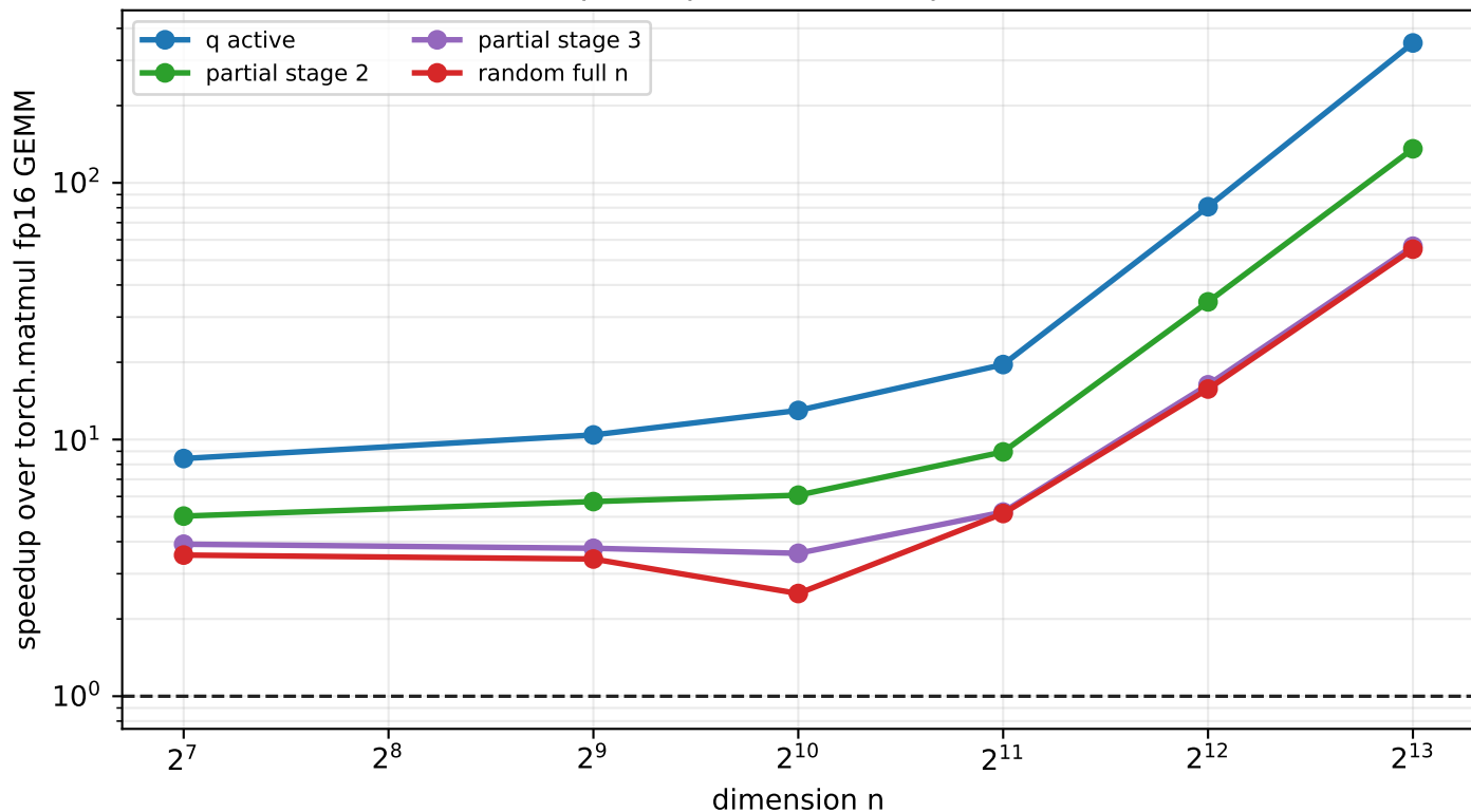
422 speedup over dense fp16 GEMM
