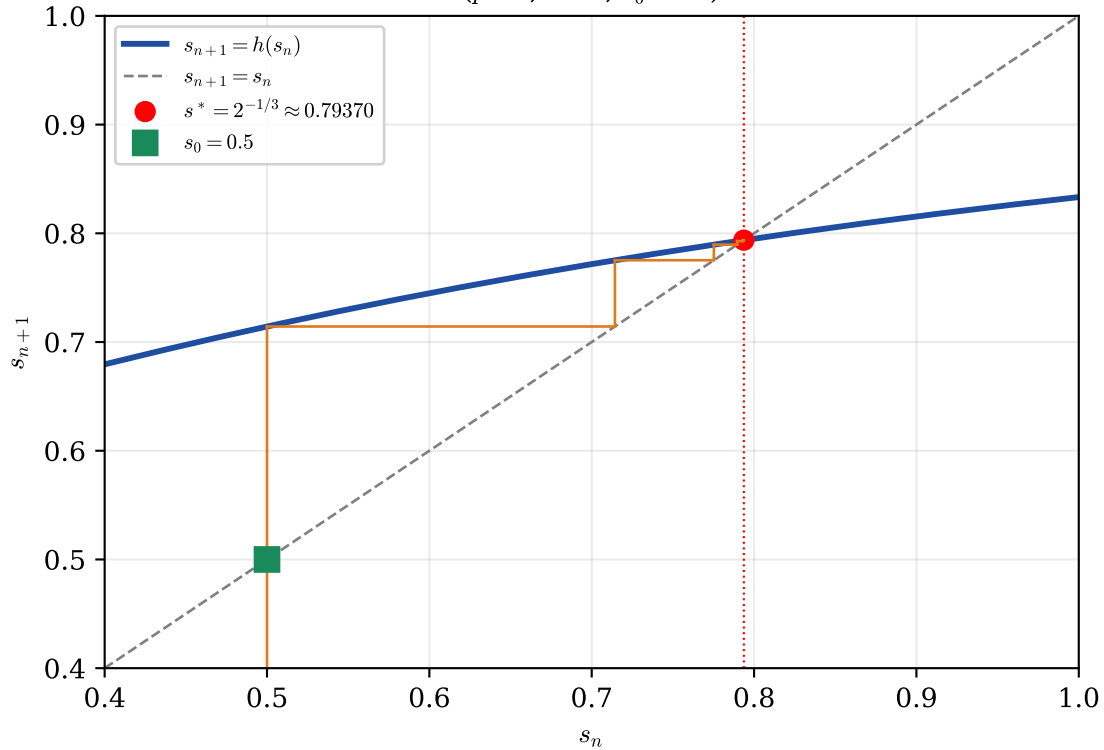
Cobweb diagram --- Pandrosion convergence (p=3, x=2, s_0=0.5)
