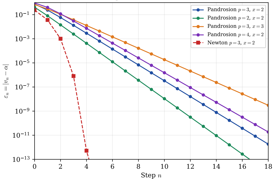
Residual profiles: Pandrosion vs Newton
