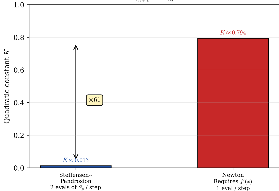
Quadratic constant comparison
