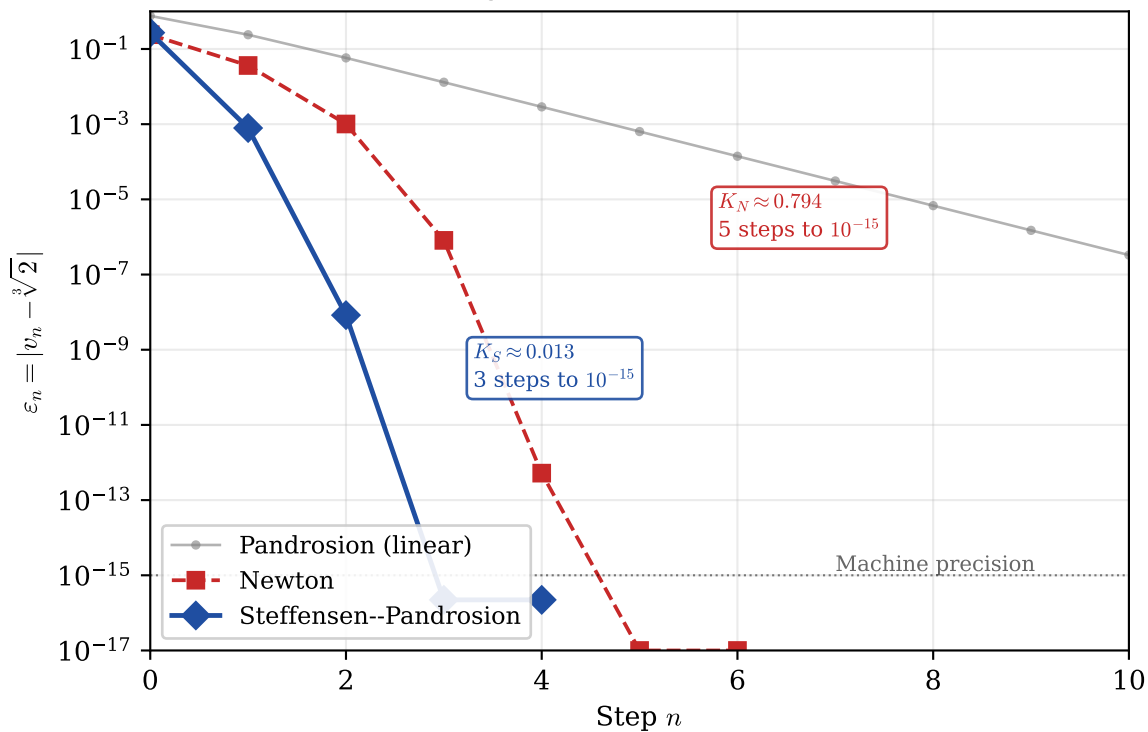
Convergence comparison ( p = 3, x = 2 )
