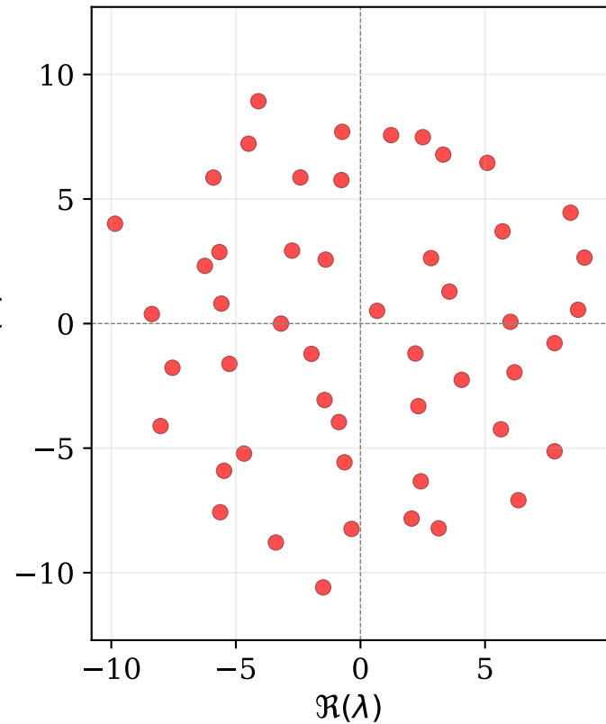
Generic Operator Eigenvalues scatter across \mathbb{C}
