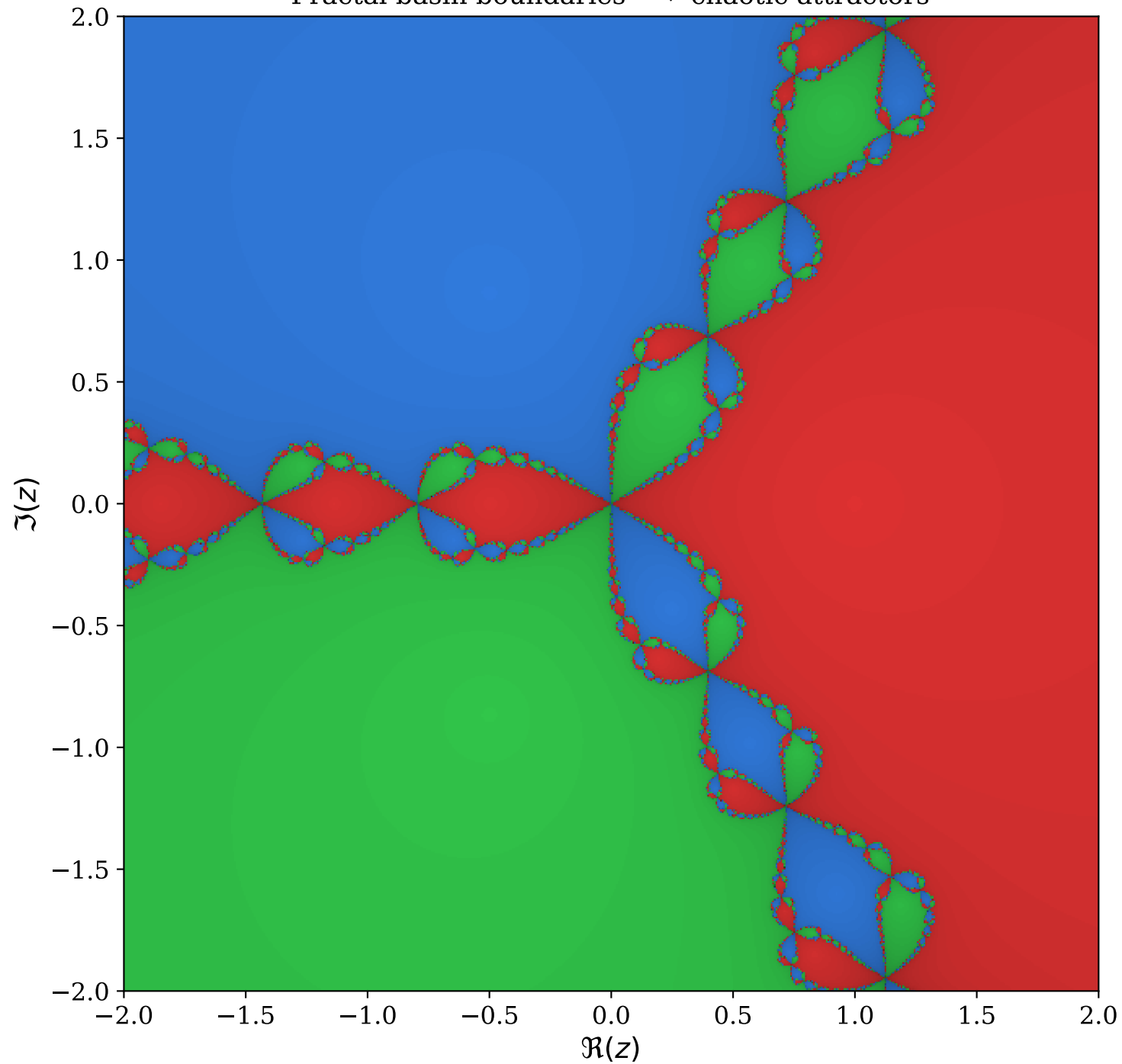
Newton's Method: z^3 - 1 Fractal basin boundaries \rightarrow chaotic attractors
