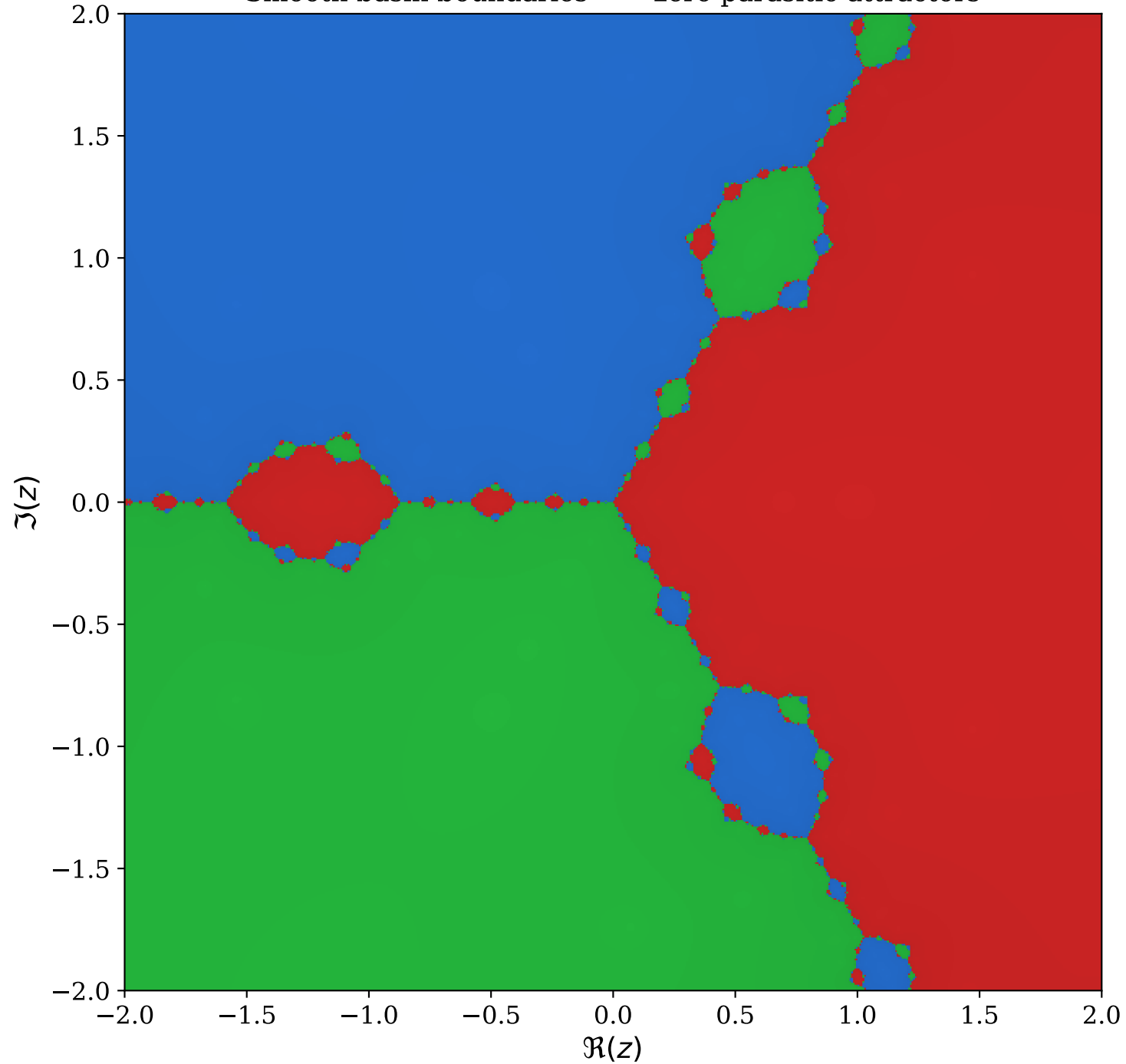
Pandrosion Iteration: z^3 - 1 Smooth basin boundaries \rightarrow zero parasitic attractors
