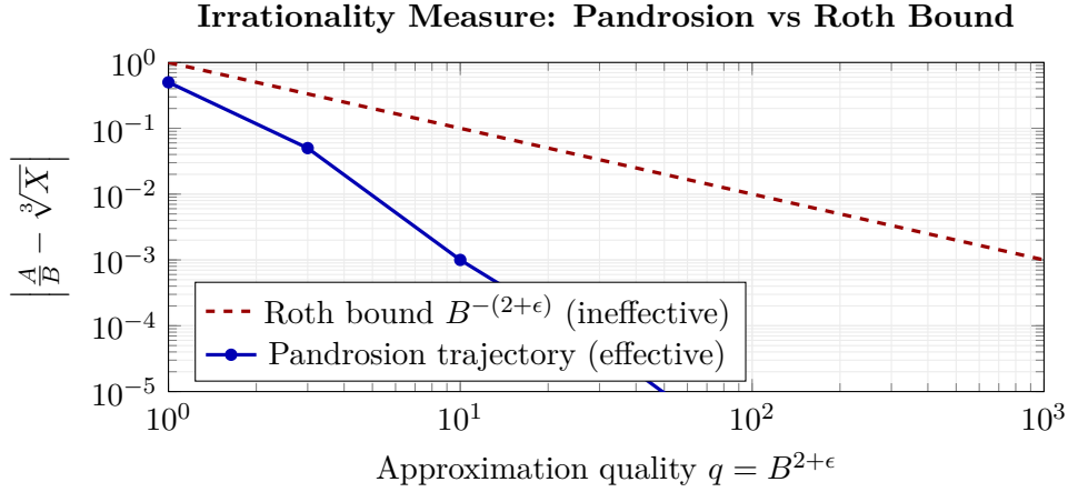
Figure 20: Effective vs Roth bound (schematic). The classical Roth bound (red dashed) guarantees existence but provides no constructive rate. The Pandrosion sequence (blue) achieves an explicit algebraic recurrence within its own iterates . This does not constitute a general effective irrationality measure; it is a property of this specific fractional progression.
