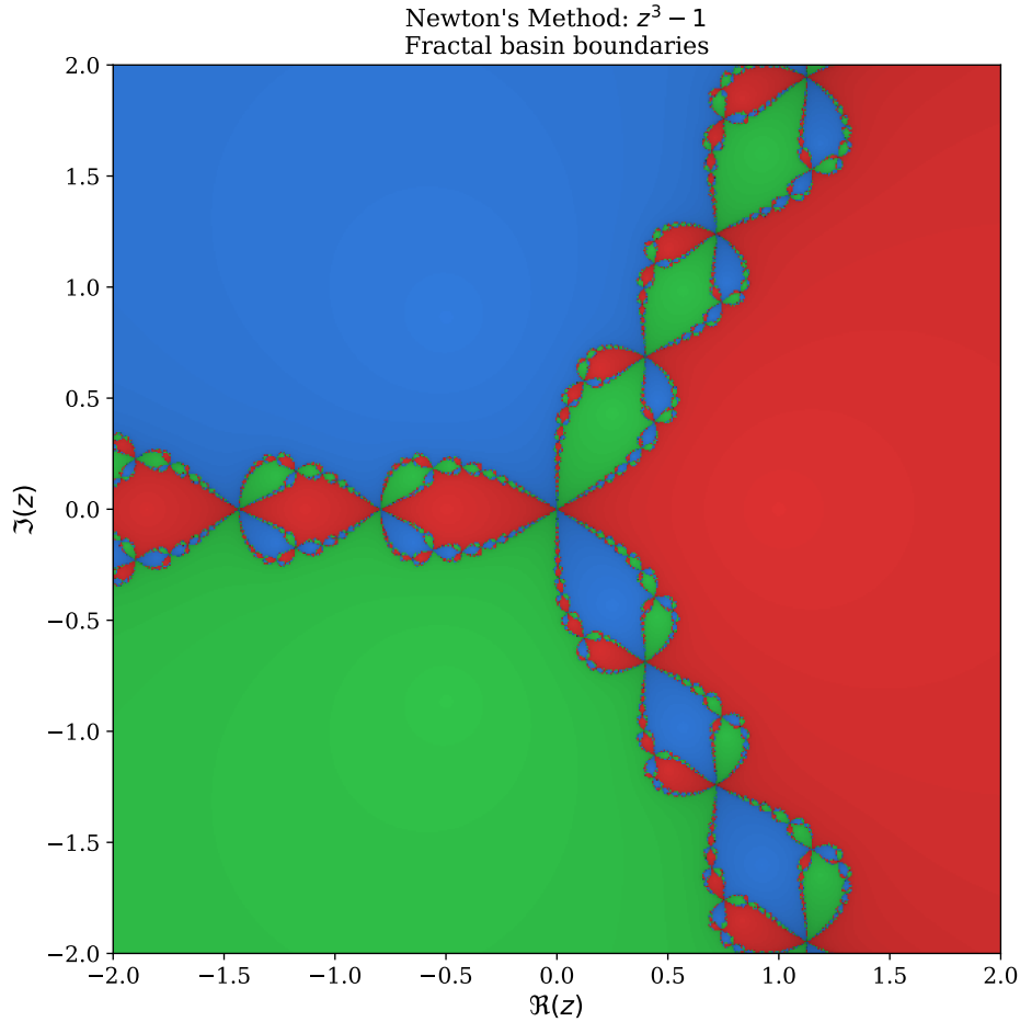
Figure 9: Newton’s method fractal for z^3 - 1 on \mathbb{C} . The three attraction basins (red, blue, green) are separated by infinitely intricate fractal boundaries — the Julia set. Points near these boundaries undergo chaotic, unpredictable iterations, creating parasitic computational traps. This fractal complexity is the hallmark of derivative-based root-finding in the complex plane.
