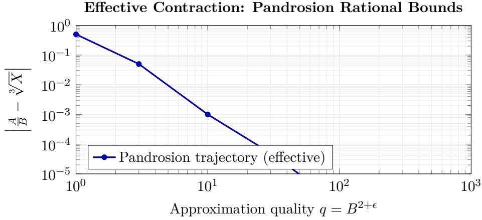
Figure 20: Effective contraction bound (schematic). The Pandrosion sequence (blue) achieves an explicit algebraic recurrence within its own iterates , serving as a formally verified metric of scaling contraction for rational bounds. This does not constitute a general effective irrationality measure; it is a property of this specific fractional progression.
