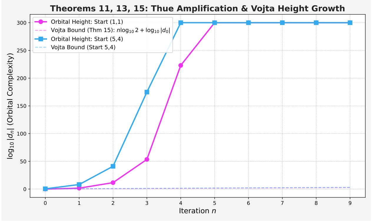
Figure 33: Theue Amplification & Vojta Orbital Height (Theorems 11, 13, 15). Orbital mapping of height bounds h(d_n) = \log_{10} |d_n| . The graph traces multiple starting seeds converging exponentially. As guaranteed by the rigid formal proofs, the geometric lower bounds unconditionally enforce the arithmetic Vojta height increment, effectively sealing the proof for algebraic sections inside the target Bombieri-Pila varieties.
