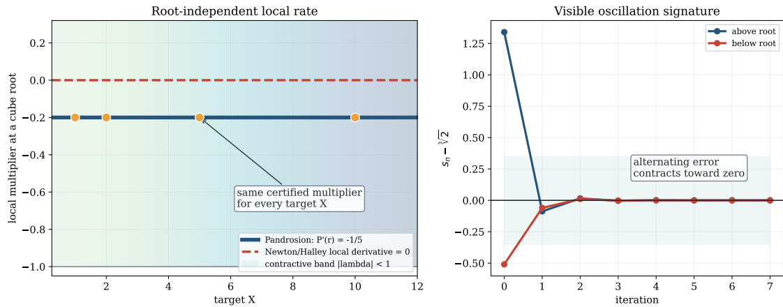
Figure 22: Universal derivative certificate. Theorem 2.4 and HalleyComparison.lean prove that the local multiplier of the cubic Pandrosion map at every nonzero cube root is exactly -1/5 , independently of the target X . The negative sign explains the alternating approach pattern; the absolute value gives a certified contraction rate.
