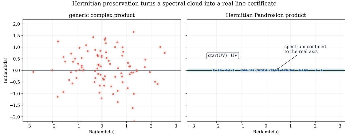
Figure 29: Hermitian preservation. Theorem 7.2 and HermitianPreservation.lean prove that the Pandrosion numerator and denominator product preserves the Hermitian condition when the inputs are Hermitian and commute. The visual consequence is spectral confinement to the real axis, unlike a generic complex product.
