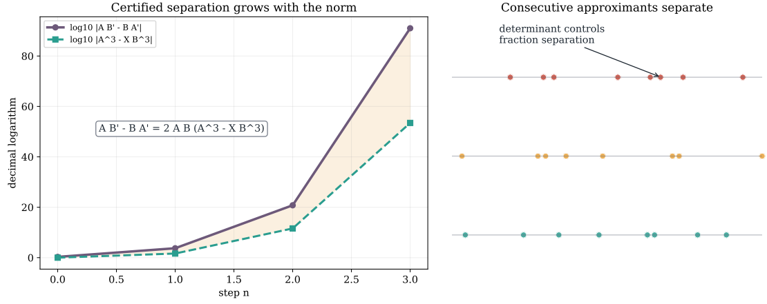
Figure 27: Cross-determinant separation. Theorem 6.2 proves AB' - BA' = 2AB(A^3 - XB^3) . This locks the separation of consecutive rational approximants to the same cubic norm that drives the Thue-style amplification, so distinctness is carried by an explicit polynomial certificate.
