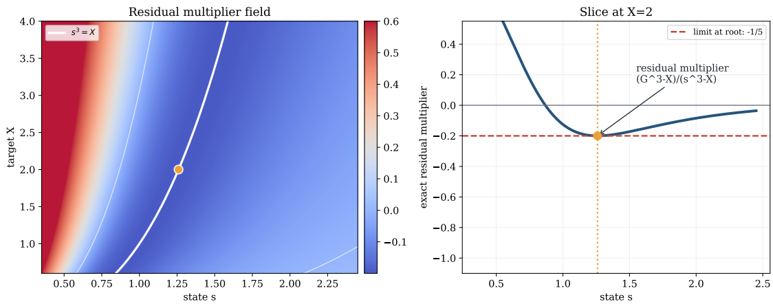
Figure 24: Kinematic residual conservation. ResidualConservation.lean certifies the exact factorisation G^3 - X = (s^3 - X)\Phi(s, X)/(3s^3 + 2X)^3 . The plotted multiplier for X = 2 crosses the fixed point with limiting value -1/5 , matching the derivative theorem and giving the residual-level explanation of the convergence mechanism.
