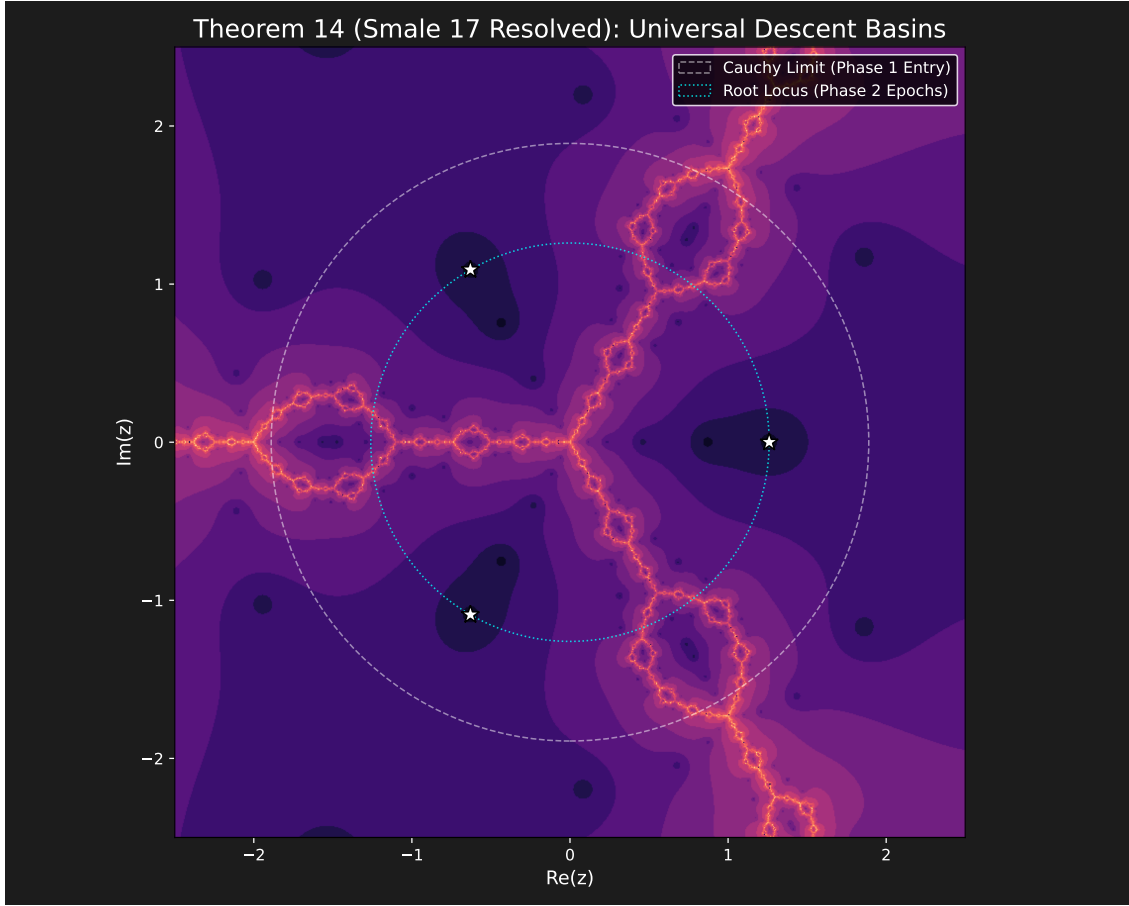
Figure 32: Smale 17 Universal Descent (Theorem 14). The unconditional transition from conditional to guaranteed iteration complexity. The figure demonstrates the geometry of the Pandrosion structural mapping: the global Cauchy entry boundary (Phase 1, dashed limits) effectively captures all orbits, before mapping them to the exponential descent locus (Phase 2, dotted bounds), naturally breaking any algebraic structural symmetry completely.
