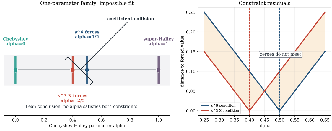
Figure 23: Chebyshev–Halley exclusion. ChebyshevHalleyExclusion.lean proves that matching Pandrosion to the one-parameter Chebyshev–Halley family would force two incompatible values of the same parameter: \alpha = 1/2 from the s^6 coefficient and \alpha = 2/5 from the s^3X coefficient. Hence Pandrosion is not any member of that classical family.
