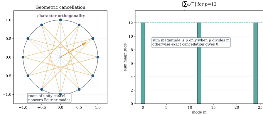
Figure 30: DFT character orthogonality. DFTDecomposition.lean proves the roots-of-unity cancellation law: \sum_{j=0}^{p-1} \omega^{jm} is p when p \mid m and 0 otherwise. This supplies the spectral bookkeeping used by the Fourier and descent modules.
