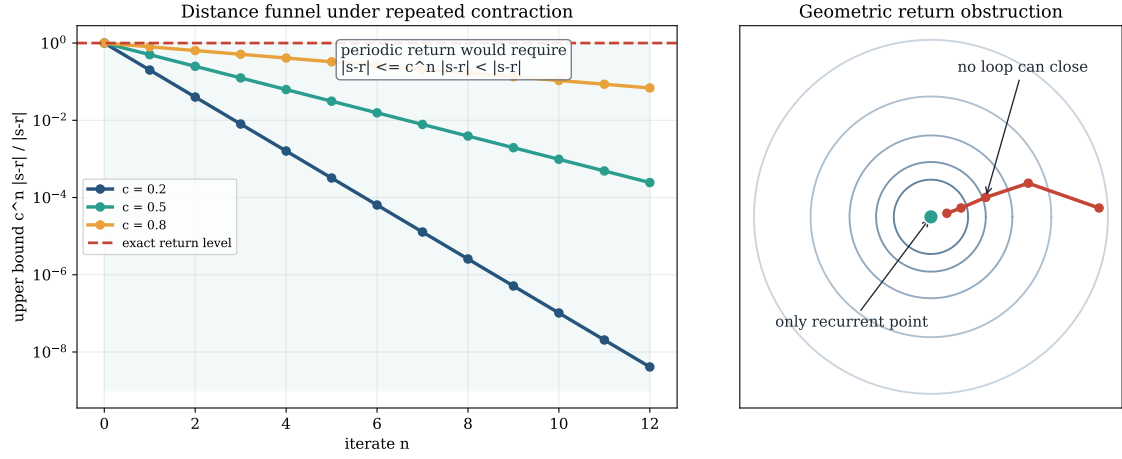
Figure 25: No periodic orbits under contraction. NoCycles.lean proves that if |f(s) - r| \leq c|s - r| with 0 \leq c < 1 , then any finite periodic return f^{c^n}(s) = s forces s = r . The figure shows why: every composed contraction multiplies the nonzero distance by c^n < 1 , contradicting exact return.
