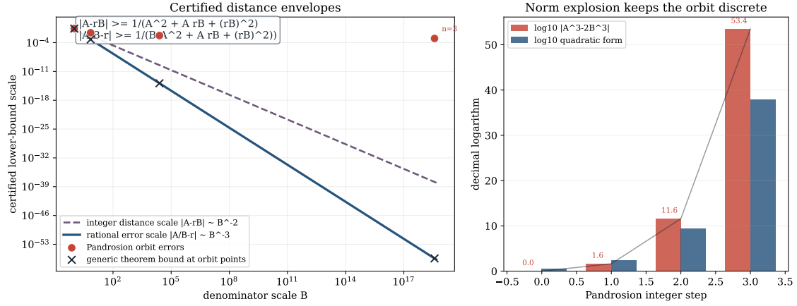
Figure 31: Effective irrationality bound. Theorem 10.1 in EffectiveIrrationality.lean turns the cubic factorisation A^3 - (rB)^3 = (A - rB)(A^2 + ArB + (rB)^2) and the discreteness of nonzero integers into an explicit lower bound for |A - rB| ; dividing by B gives the corresponding rational approximation bound for |A/B - r| . The Pandrosion norm propagation keeps this bound applicable along the integer orbit.
