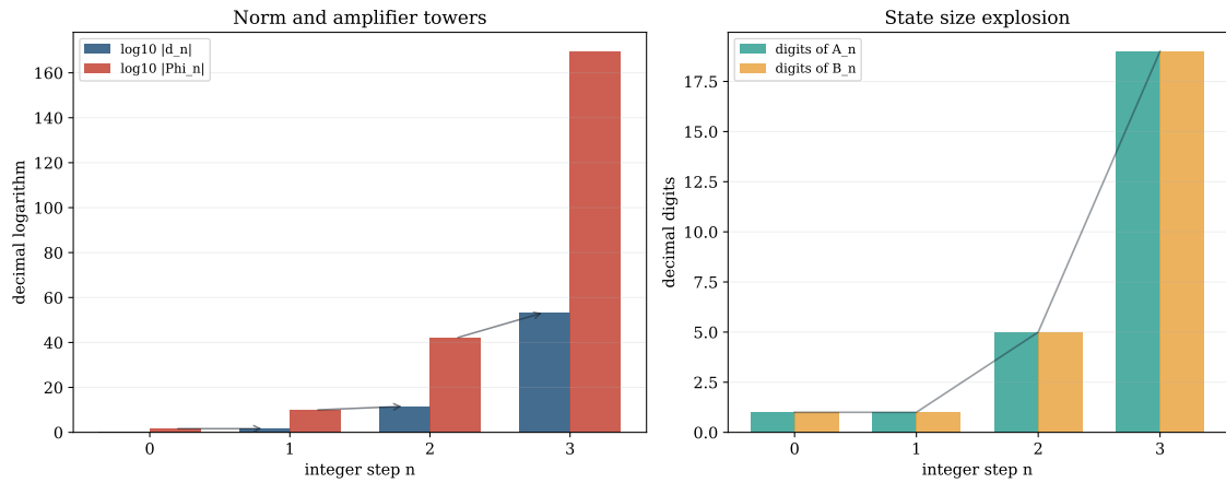
Figure 26: Pell–Pandrosion integer amplification. Theorem 4.1 and ThueBridge.lean prove the exact law d_{n+1} = d_n \Phi_n for d_n = A_n^3 - X B_n^3 . For X = 2 , the logarithmic growth of both the norm and the amplification factor becomes enormous after only a few certified integer steps.
