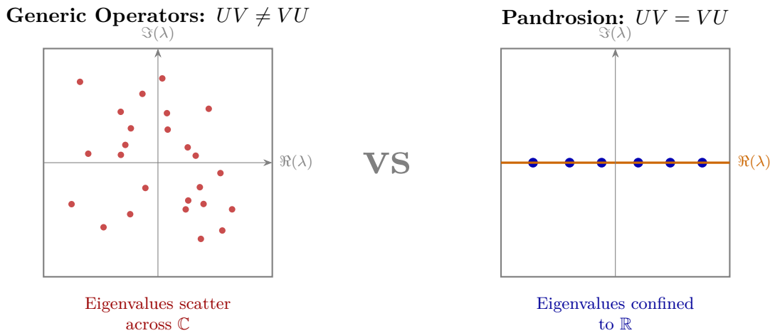
Figure 16: Commutativity and spectral structure (schematic) . Left: For generic non-commuting operators, eigenvalues of UV are distributed across \mathbb{C} . Right: When U, V commute (as proven in Deep 30), they share an eigenbasis; combined with Hermitian inputs, this confines eigenvalues to \mathbb{R} .
