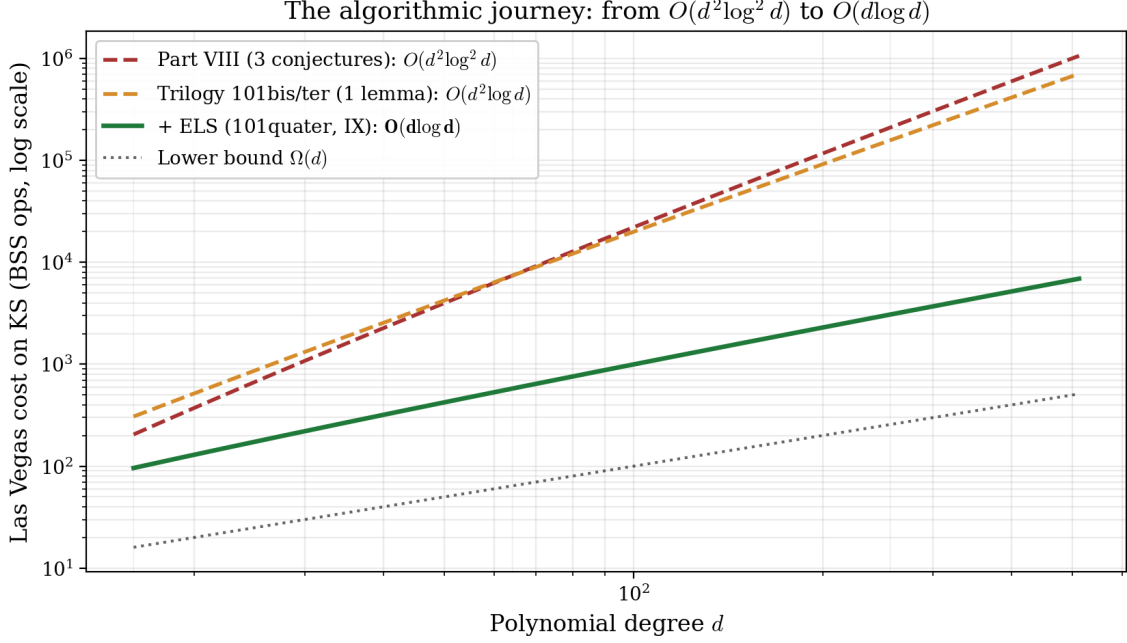
Figure 2: The algorithmic journey on KS over d \in [16, 512] : from Part VIII’s O(d^2 \log^2 d) (red dashed, conditional on three conjectures) to the trilogy’s O(d^2 \log d) (orange, conditional on one lemma) to ELS’s O(d \log d) (green, conditional on two lemmas), within \log d of the trivial lower bound \Omega(d) (black dotted).
