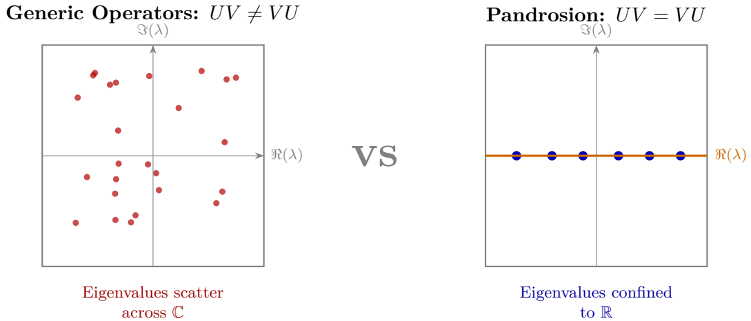
Figure 16: Commutativity and spectral structure (schematic) . Left : For generic non-commuting operators, eigenvalues of UV are distributed across \mathbb{C} . Right : When U, V commute (as proven in Deep 30), they share an eigenbasis; combined with Hermitian inputs, this confines eigenvalues to \mathbb{R} .
