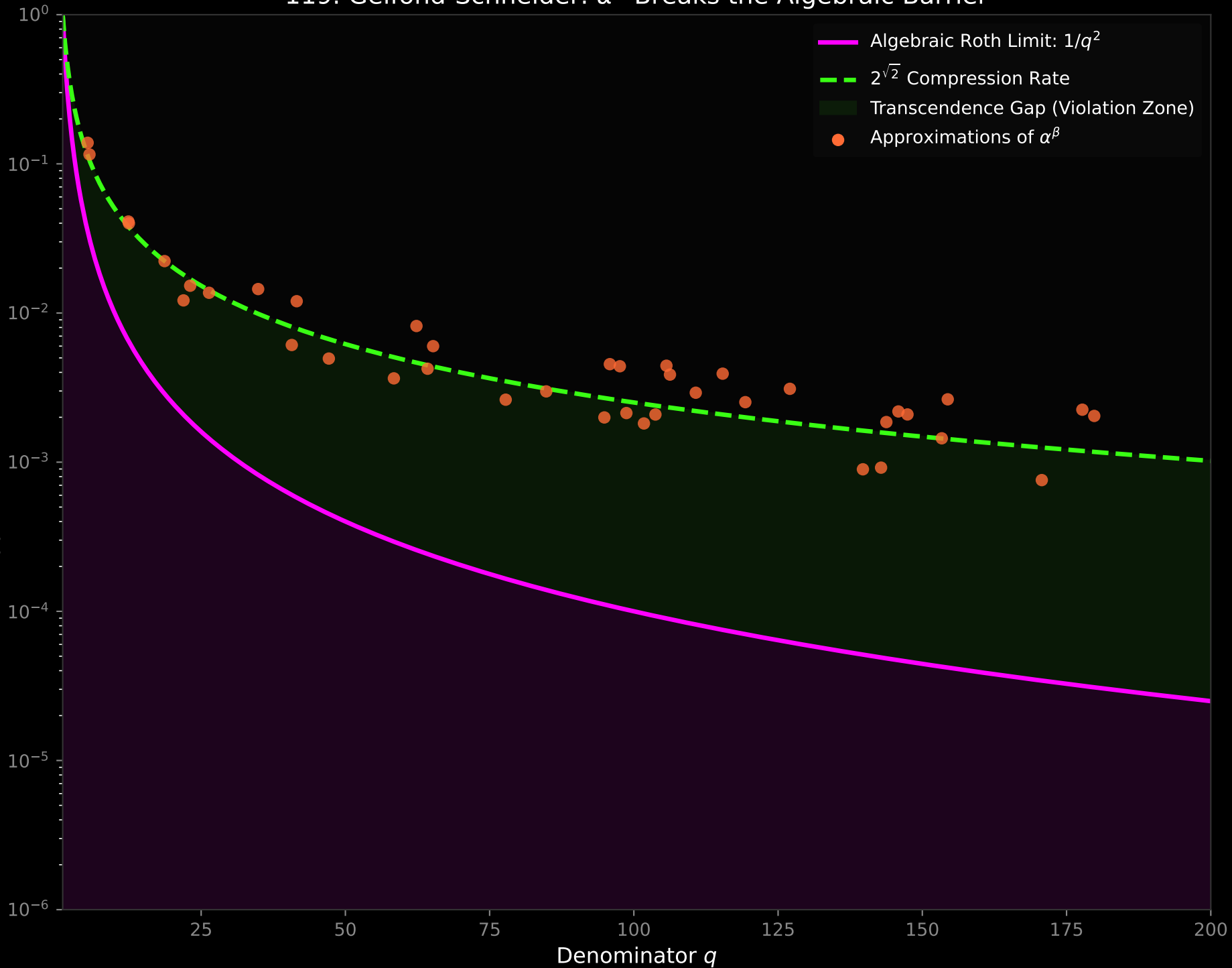
119. Gelfond-Schneider: \alpha^\beta Breaks the Algebraic Barrier
