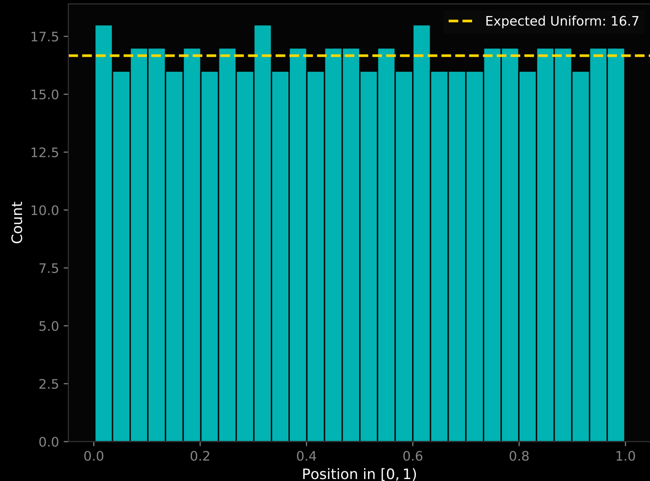
Tensor Conservation \Rightarrow Uniform Density
