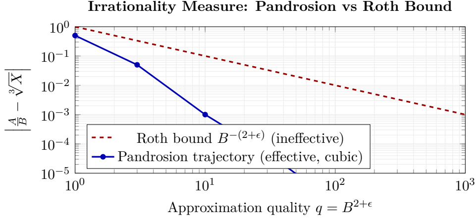
Figure 20: Effective vs ineffective irrationality bounds. The classical Roth bound (red dashed) guarantees existence but provides no constructive rate. The Pandrosion trajectory (blue) achieves explicit cubic contraction, making the irrationality measure fully effective .
