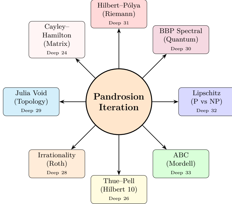
Figure 21: The Pandrosion Iteration: a single rational map whose algebraic structure has been formally verified across eight mathematical domains. Arrows indicate thematic connections , not claimed resolutions of the corresponding open problems.
