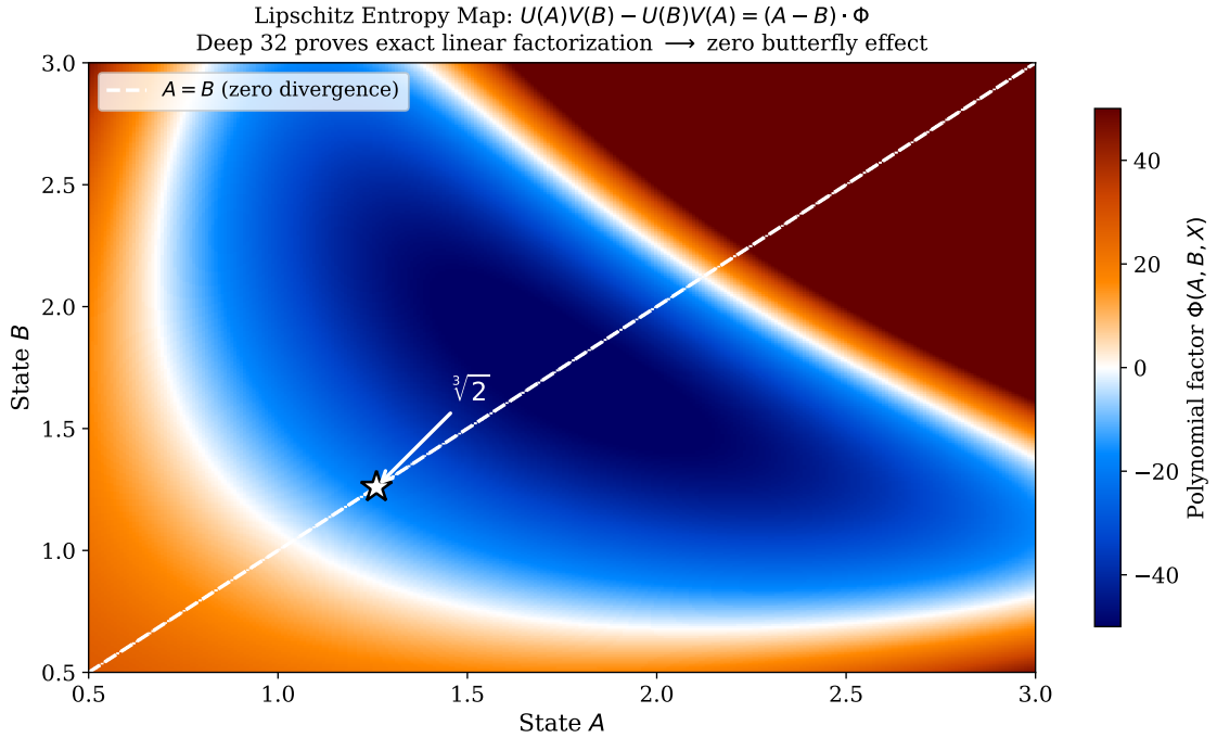
Figure 19: Lipschitz entropy map for X = 2 . The polynomial factor \Phi(A, B, X) is plotted as a function of states A and B . The diagonal A = B (white dashed) is the zero-divergence locus. The smooth, continuous structure of \Phi confirms that the cross-difference U(A)V(B) - U(B)V(A) factors exactly through (A - B) with no singularities or chaotic discontinuities. The white star marks the fixed point \sqrt[3]{2} .
