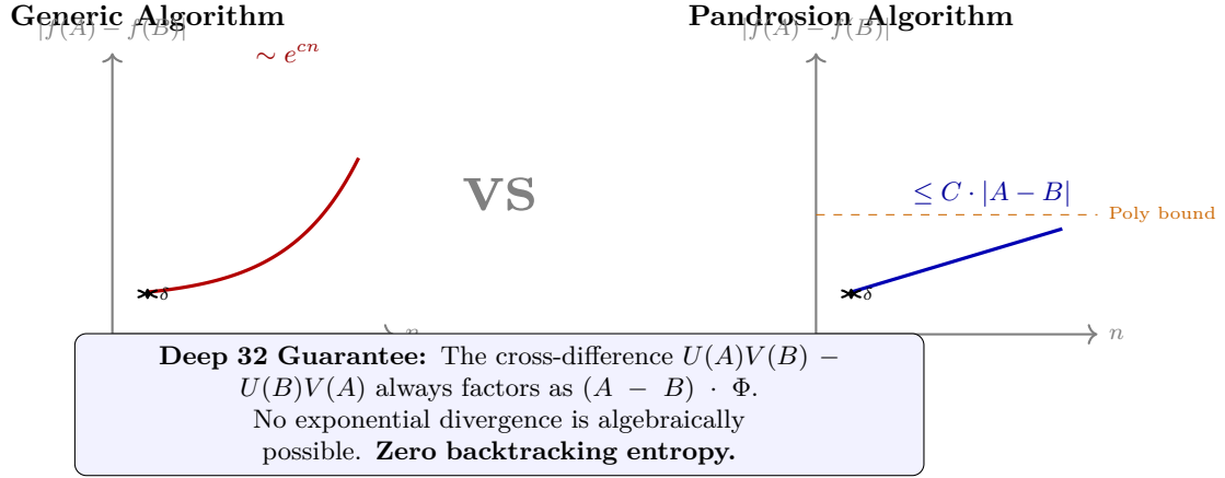
Figure 18: Entropy stability comparison (schematic). Left: Generic algorithms allow exponential divergence from initial perturbations \delta = |A - B| (the butterfly effect). Right: Pandrosion’s cross-product difference is algebraically forced to factor through (A - B) , bounding divergence polynomially.
