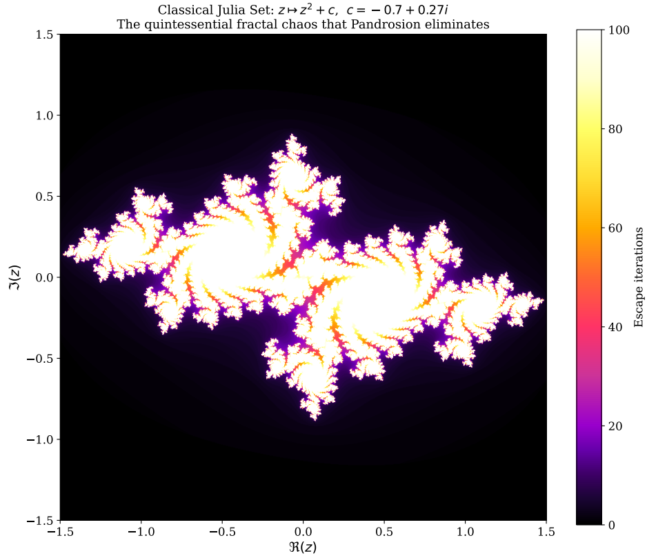
Figure 11: Classical Julia Set for z \mapsto z^2 + c with c = -0.7 + 0.27i . This iconic fractal illustrates the fundamental complexity barrier in iterative dynamics on \mathbb{C} : the boundary between convergent and divergent orbits is infinitely intricate. The Universitas Pandrosion framework (Deep 29) proves that the Pandrosion map structurally cannot generate such fractal boundaries, making it topologically “sterile” by construction.
