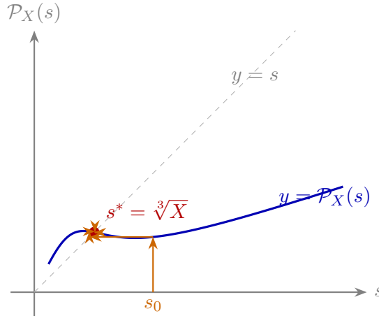
Figure 1: Cobweb diagram for X = 2 . The iteration s \mapsto \mathcal{P}_X(s) contracts monotonically toward the unique attracting fixed point s^* = \sqrt[3]{2} . No parasitic cycles exist (Theorem 2.2).
