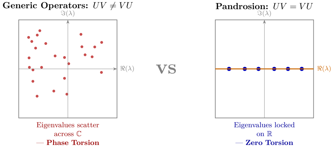
Figure 14: Spectral Phase Locking (schematic) . Left: Generic non-commuting operators scatter eigenvalues chaotically across \mathbb{C} . Right: The Pandrosion operators U, V are proven to commute (Deep 30), locking their shared eigenvalues onto structured spectral lines.
