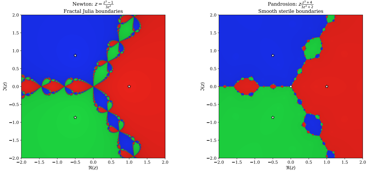
Figure 9: High-resolution side-by-side comparison. Left: Newton's method for z^3 - 1 creates intricate fractal filaments at every basin boundary, where nearby starting points can converge to entirely different roots. Right: The Pandrosion iteration for the same polynomial produces clean, smooth boundaries with zero fractal structure. White stars mark the three cube roots of unity.
