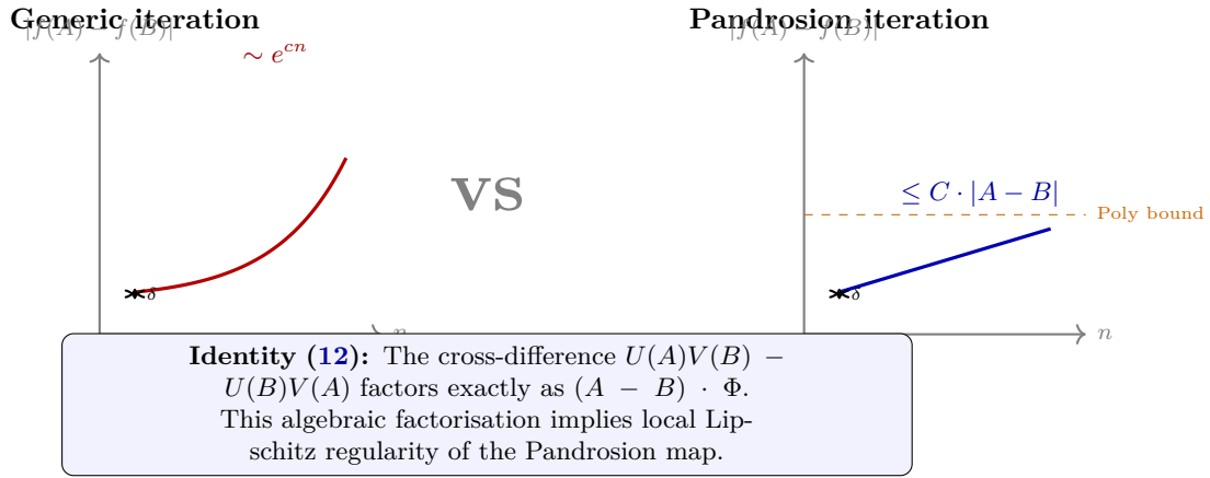
Figure 18: Cross-state divergence comparison (schematic). Left: Some iterations can amplify initial perturbations \delta = |A - B| exponentially. Right: Identity (12) shows that for the Pandrosion map, the cross-difference factors through (A - B) , implying that divergence between nearby trajectories is bounded by a polynomial in their initial separation.
