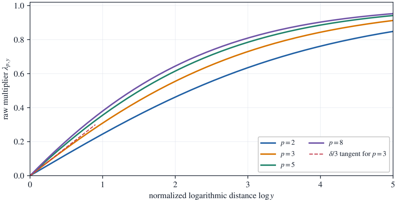
Residual fingerprint of raw Pandrosion
