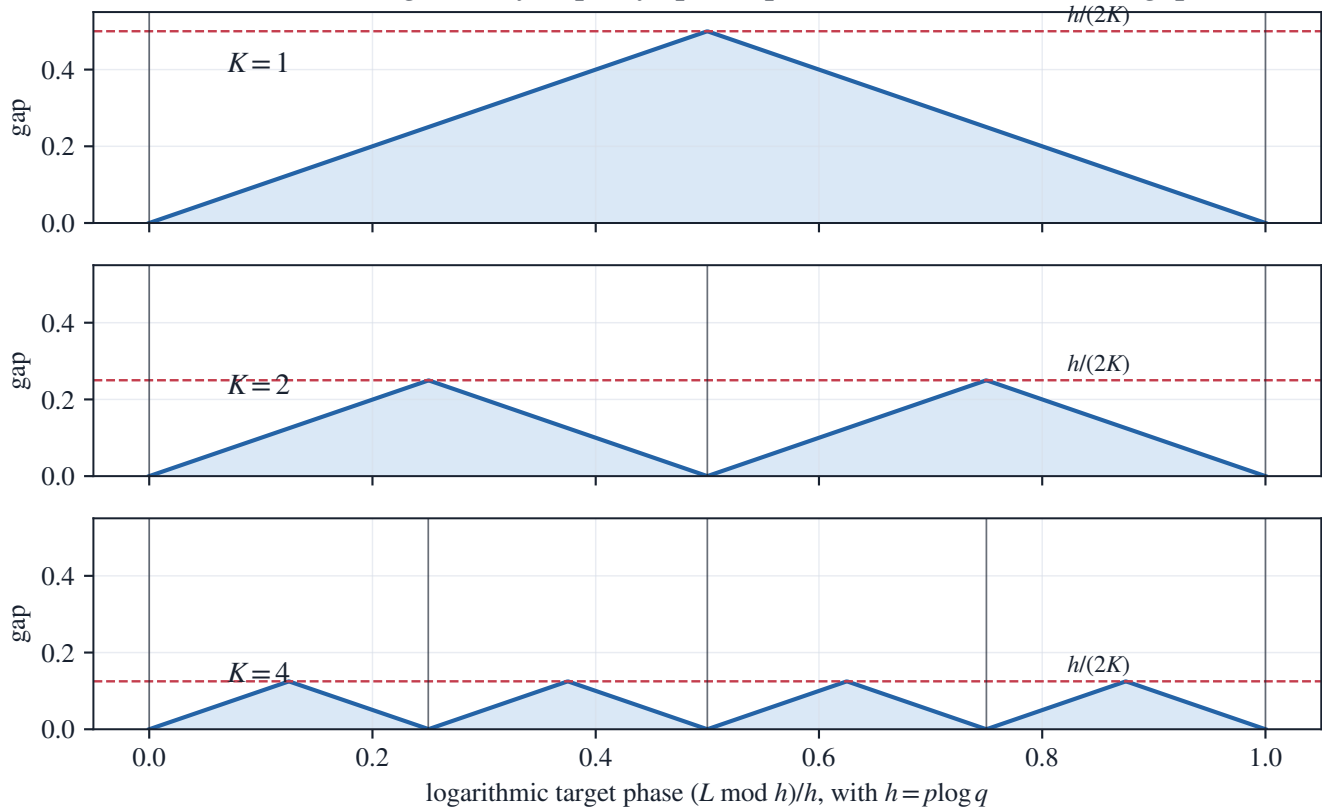
Scale-lattice geometry: equally spaced phases minimize the worst gap
