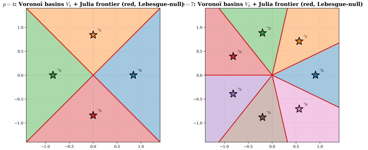
Figure 4: Voronoï decomposition of \mathbb{C} for cyclotomic anchors at p = 4 and p = 7 , x = 2 . Each colored region V_k is the basin of attraction of \gamma_k under the selector. The red frontier is what we call the Pandrosion Julia set; it is Lebesgue-null.
