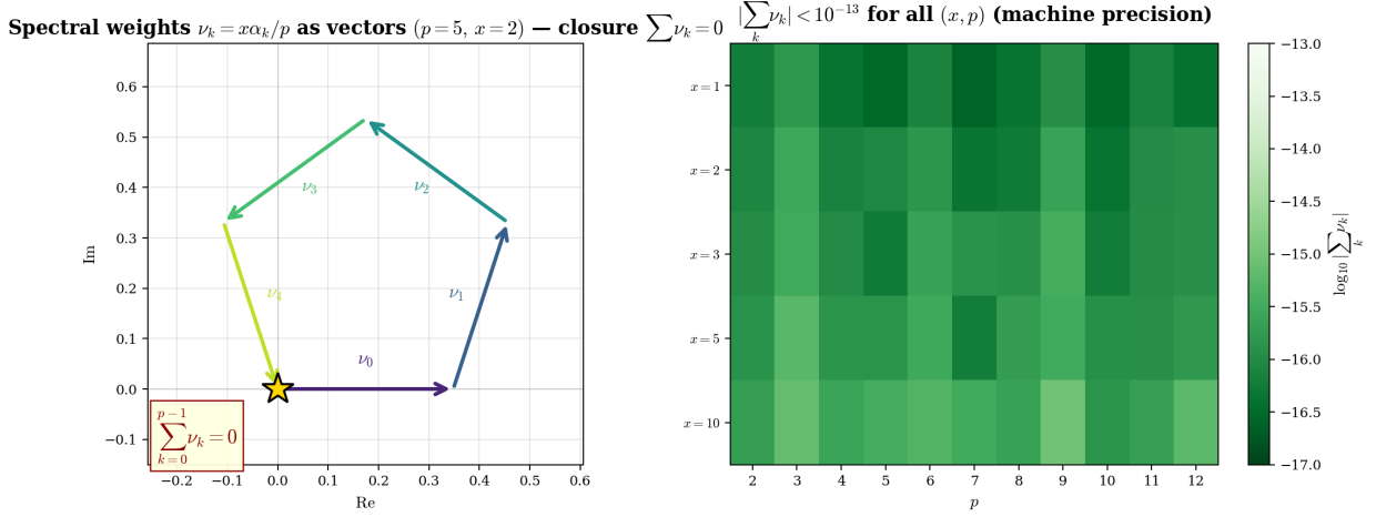
Figure 6: Left: the \nu_k as oriented vectors in \mathbb{C} for (x, p) = (2, 5) ; the head-to-tail sum closes back to the origin, visualising \sum_k \nu_k = 0 . Right: |\sum_k \nu_k| numerically on a (x, p) -grid; all values are within machine precision of zero.
