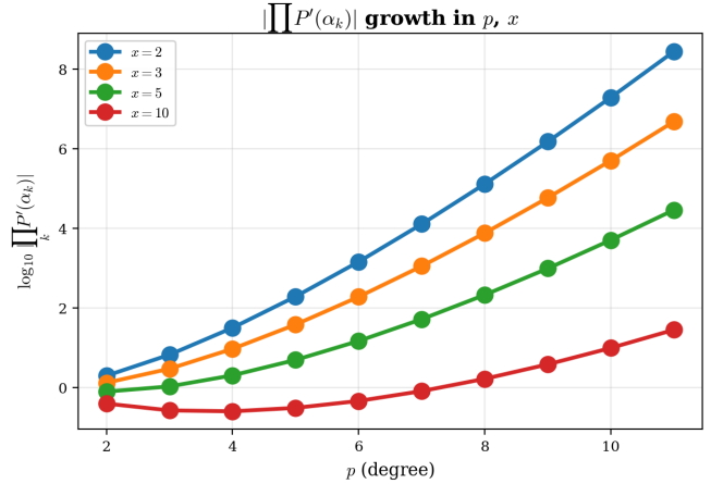
Figure 7: Numerical values of \prod_k P'(\alpha_k) matching the closed-form of Proposition 5.3 exactly; and its log-scale growth in p for fixed x .
