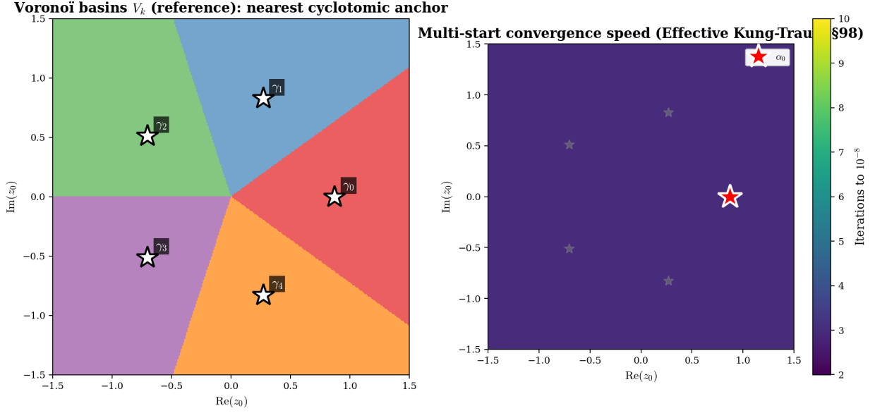
Figure 5: Left: Voronoï basins as the structural reference, computed from the nearest-anchor criterion only (no dynamics). Right: number of multi-start iterations needed to reach precision 10^{-8} ; it is bounded and essentially flat over the window, in line with Theorem 3.3.
