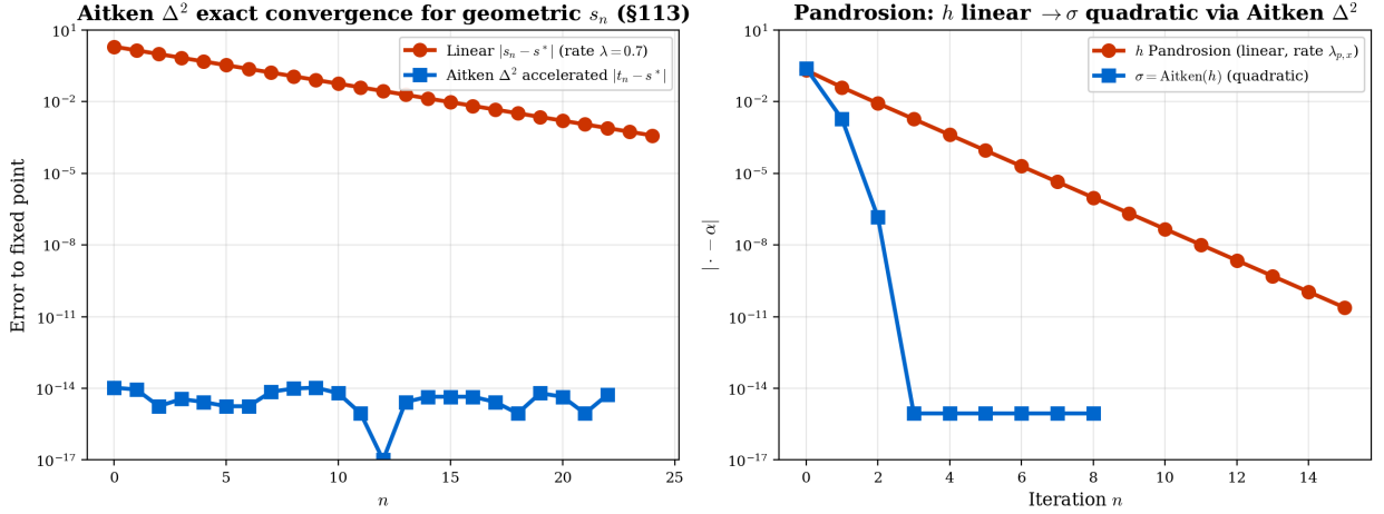
Figure 9: Left: a linearly convergent geometric sequence and its \Delta^2 -accelerated version, which collapses to s^* at machine precision. Right: h iteration (linearly convergent) vs \sigma = \text{Aitken}(h) (quadratically convergent) for (x, p) = (2, 3) , z_0 = 1 .
