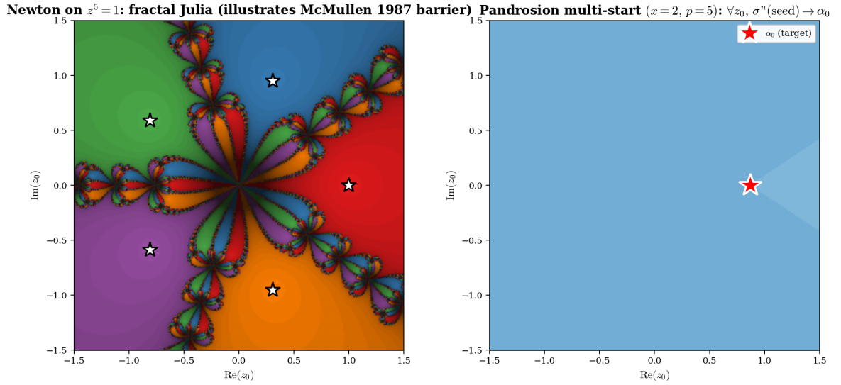
Figure 1: Left: Newton’s iteration on z^5 = 1 , coloured by which root the iteration converges to. This is the classical illustration of the kind of Julia-set obstruction that affects purely iterative root finders. Right: the Pandrosion-Steffensen multi-start scheme of this paper, coloured by the number of iterations needed to reach precision 10^{-6} from each z_0 . The seed (5) is \alpha -dependent; it is therefore not a purely iterative scheme in the sense of [17].
