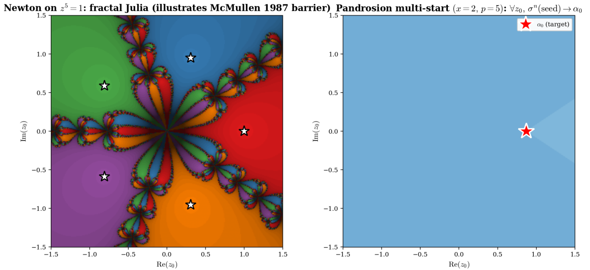
Figure 3: Structure of the multi-start seed. Each point z \in \mathbb{C} is mapped to \text{seed}_{\alpha,\varepsilon_{\text{seed}}}(z) , which lies in \overline{B}(\alpha, R_\sigma/2) regardless of z ; the iteration is then run from the seed. Colour indicates the number of iterations needed to reach precision 10^{-6} after the seed is applied. The figure illustrates how seed (9) places the scheme outside the hypotheses of [18] by making the iterate entry point \alpha -dependent; we explicitly do not compare with Newton’s basin structure here, since the two schemes do not solve the same problem (Newton is parameter-free, multi-start is \alpha -targeted).
