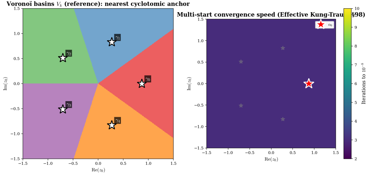
Figure 6: Left: Voronoi basins as the structural reference, computed from the nearest-anchor criterion only (no dynamics). Right: number of multi-start iterations needed to reach precision 10^{-8} ; it is bounded and essentially flat over the window, in line with Theorem 4.5.
