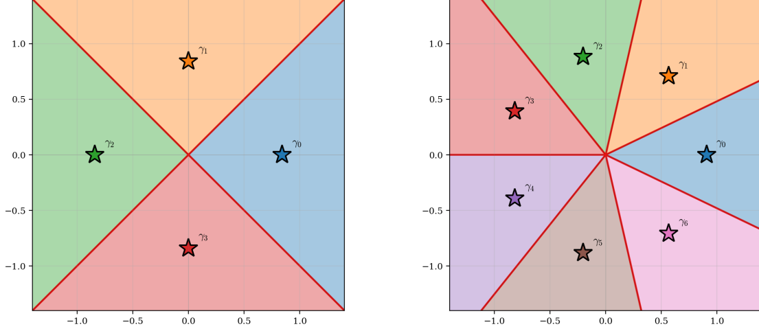
Figure 5: Voronoi decomposition of \mathbb{C} for cyclotomic anchors at p = 4 and p = 7 , x = 2 . Each colored region V_k is the basin of attraction of \gamma_k under the selector. The red frontier is the Voronoi boundary of the cyclotomic anchor set; it is Lebesgue-null.
