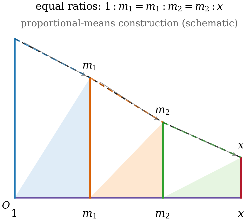
Figure 1: Proportional-means construction, with lengths not drawn to scale. The dashed parallels encode the Thales-type step, and the shaded triangles indicate the repeated similarity condition 1 : m_1 = m_1 : m_2 = m_2 : x .
