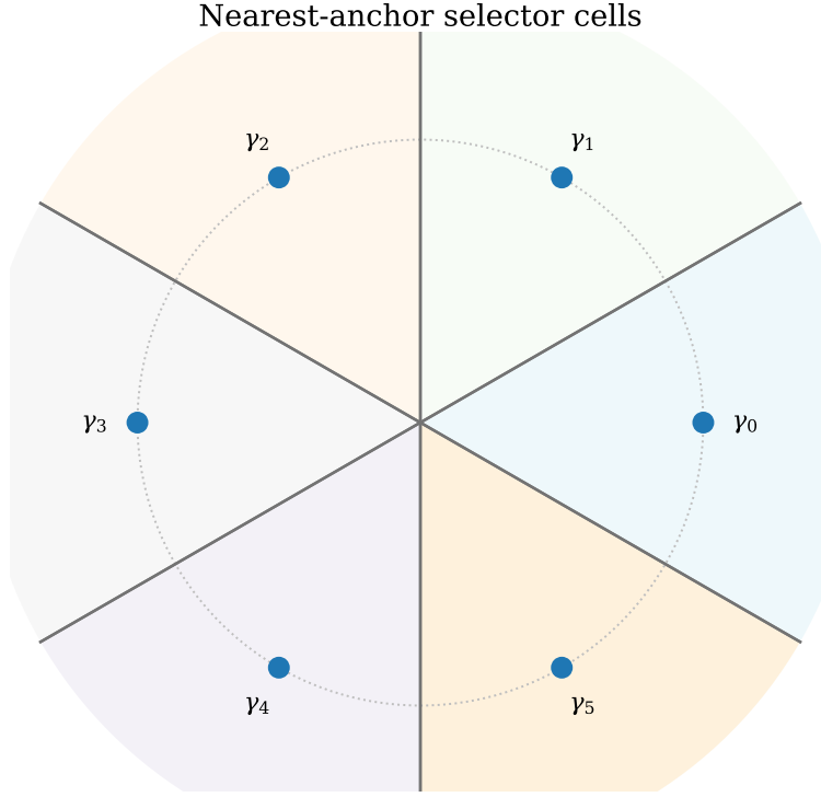
Figure 7: The nearest-anchor selector partitions the complex plane into Voronoi cells. The selector is simple and locally stable away from the cell boundaries.
