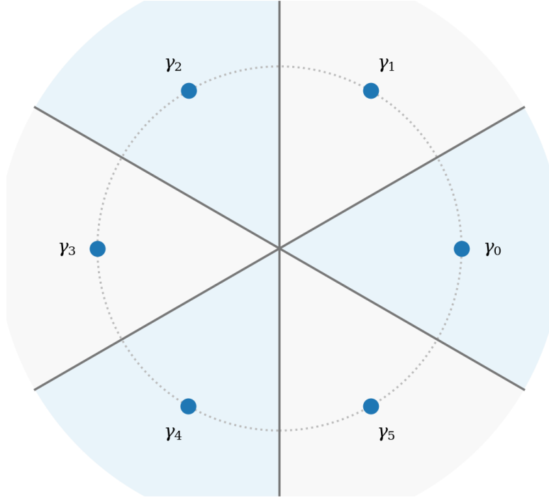
Figure 7: The nearest-anchor selector partitions the complex plane into Voronoi cells. The selector is simple and locally stable away from the cell boundaries.
