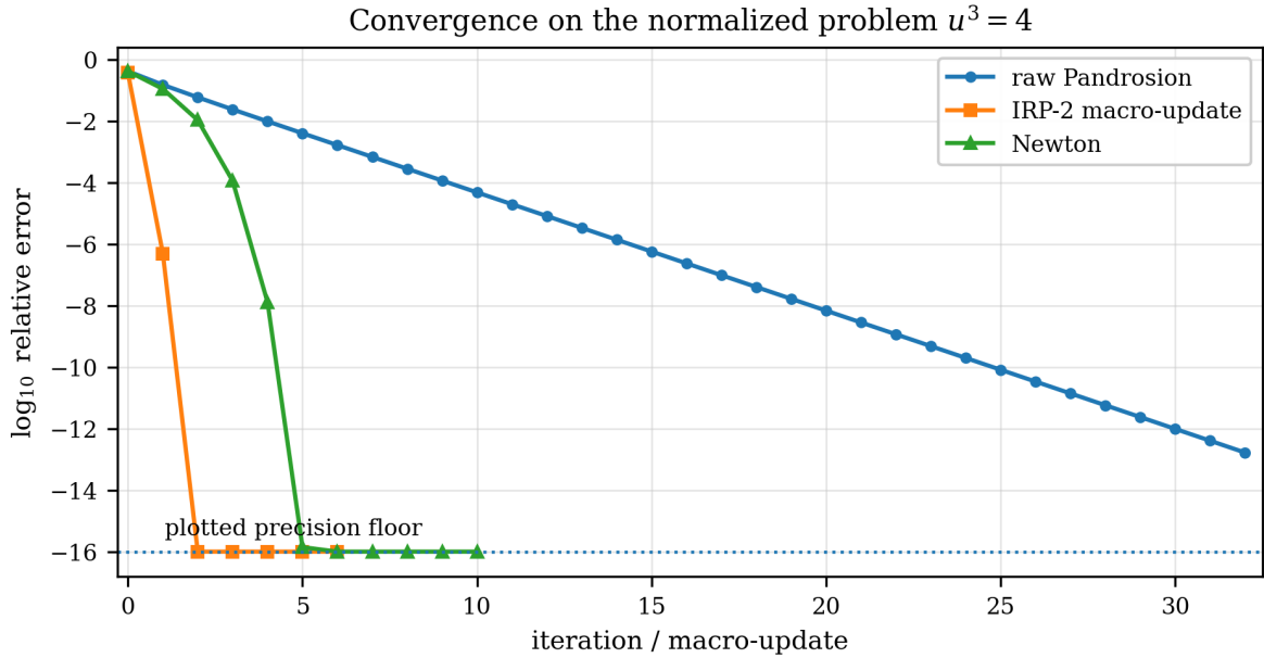
Figure 5: Iteration histories on the normalized problem u^3 = 4 . Raw Pandrosion is linear, IRP-2 collapses the residual by repeated renormalized raw layers, and Newton provides the standard quadratic baseline; the accelerated curves are truncated once they reach the plotted precision floor.
