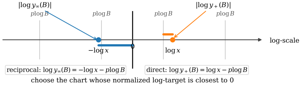
Figure 3: Direct and reciprocal logarithmic charts. The affine chart uses \log y_+(B) = \log x - p \log B , while the reciprocal chart uses \log y_\infty(B) = -\log x - p \log B . Chart selection chooses the line whose normalized logarithmic target lies closest to 0.
