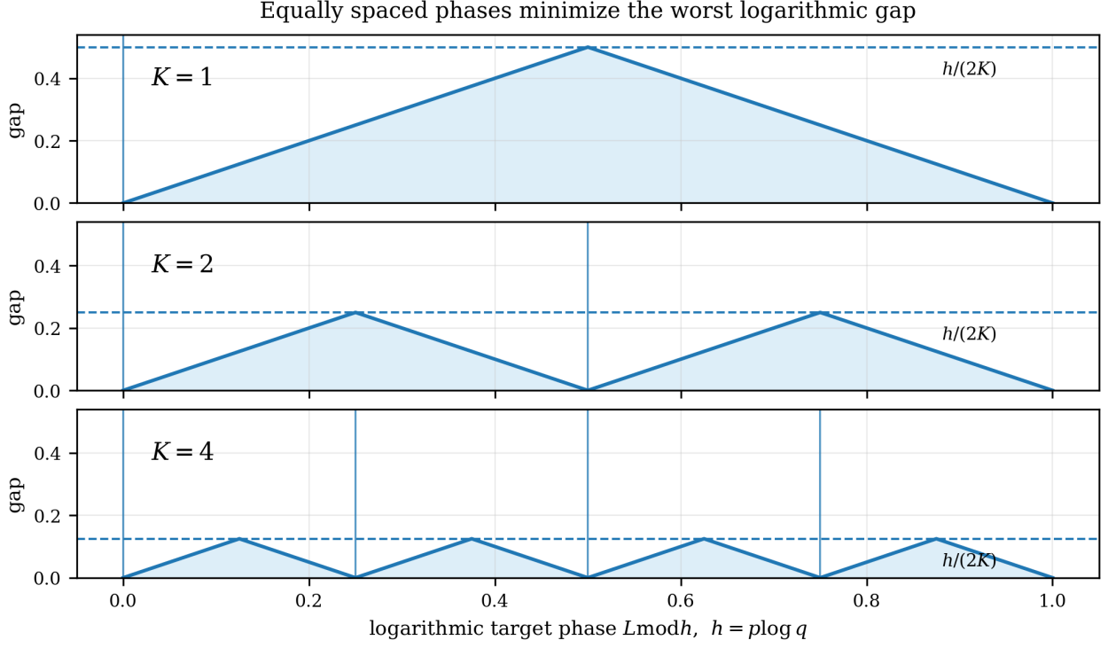
Figure 4: The scale-lattice theorem in one picture. For a logarithmic period h = p \log q , equally spaced K -phase palettes have covering radius h/(2K) , and no K -point palette can do better.
