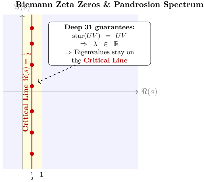
Figure 16: The Hilbert–Pólya connection. The Riemann Hypothesis asserts that non-trivial zeros of \zeta(s) lie on the critical line \Re(s) = \frac{1}{2} . Deep 31 proves that the Pandrosion operator UV is Hermitian, forcing all its eigenvalues onto \mathbb{R} — a concrete realization of the Hilbert–Pólya postulate.
