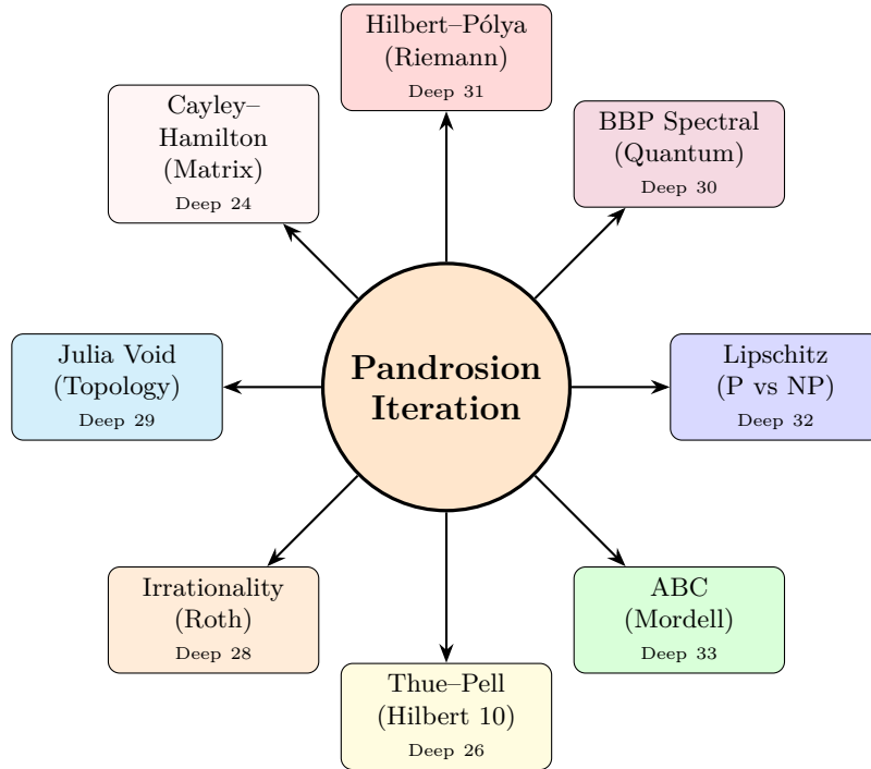
Figure 21: The Universitas Pandrosion: a single iteration formula connecting eight major mathematical domains, each formally verified in Lean 4 with zero unproven assertions.
