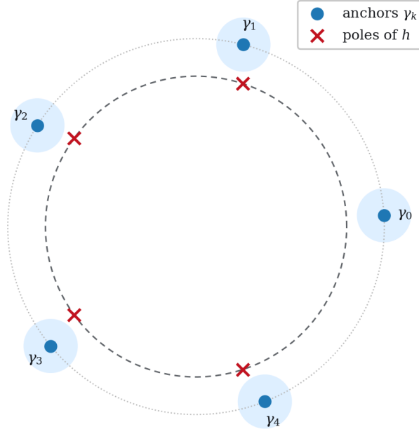
Figure 6: Cyclotomic anchors for the complex monomial problem. The poles are the non-trivial roots of unity; small disks around anchors provide local seeding regions for the accelerated map.
