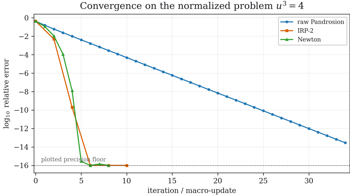
Figure 5: Iteration histories on the normalized problem u^3 = 4 . Raw Pandrosion is linear, IRP-2 collapses the residual by repeated renormalized raw layers, and Newton provides the standard quadratic baseline; the accelerated curves are truncated once they reach the plotted precision floor.
