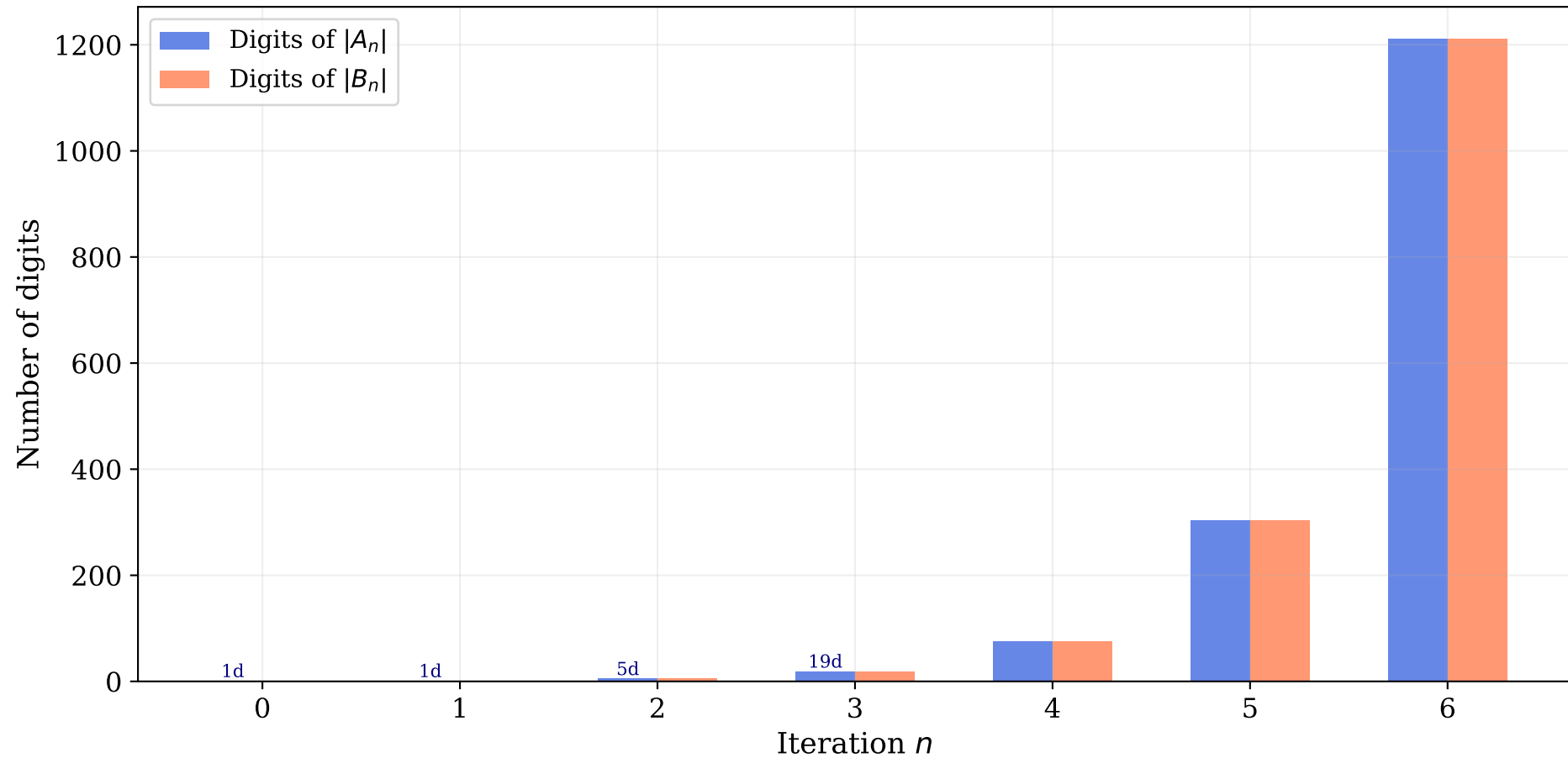
Digit growth of (A_n, B_n) for X = 2 Each step approximately cubes the digit count
