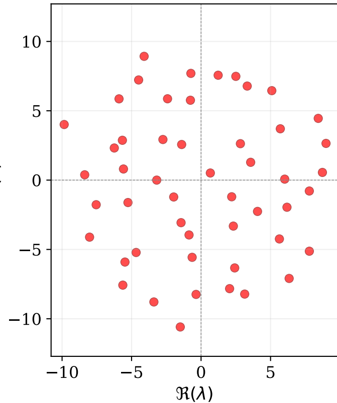
Generic Operator Eigenvalues scatter across \mathbb{C}
