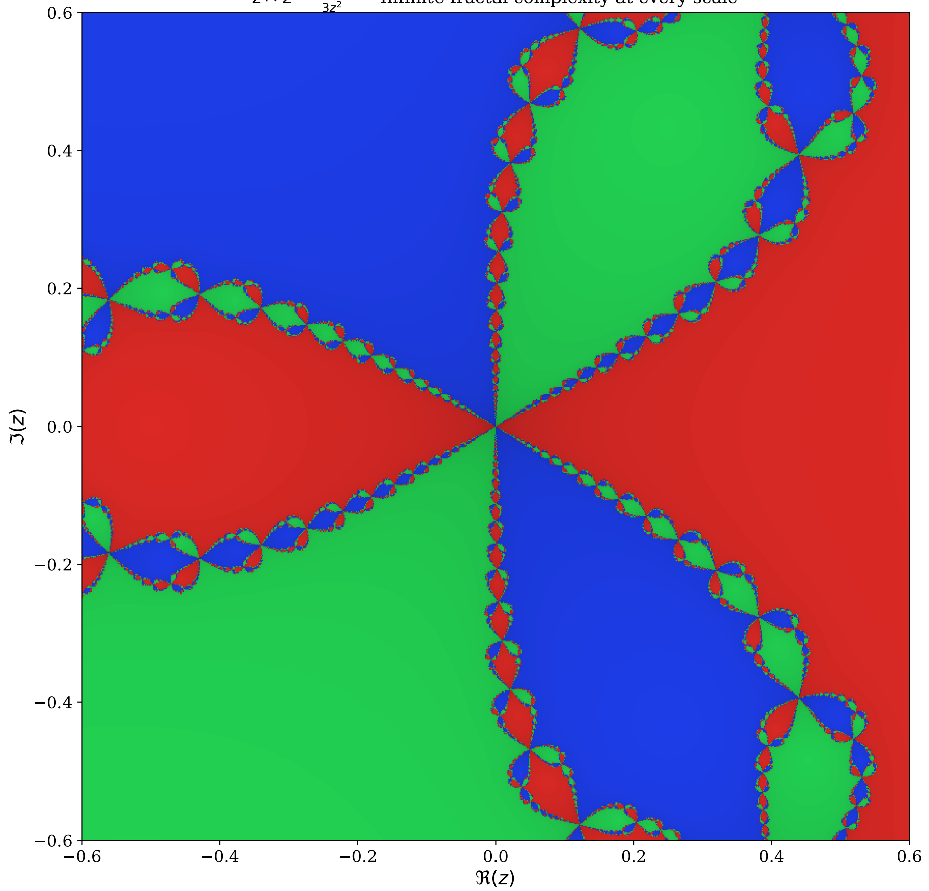
Newton's Method: Zoomed Julia Set Boundary z \mapsto z - \frac{z^3 - 1}{3z^2} — Infinite fractal complexity at every scale
