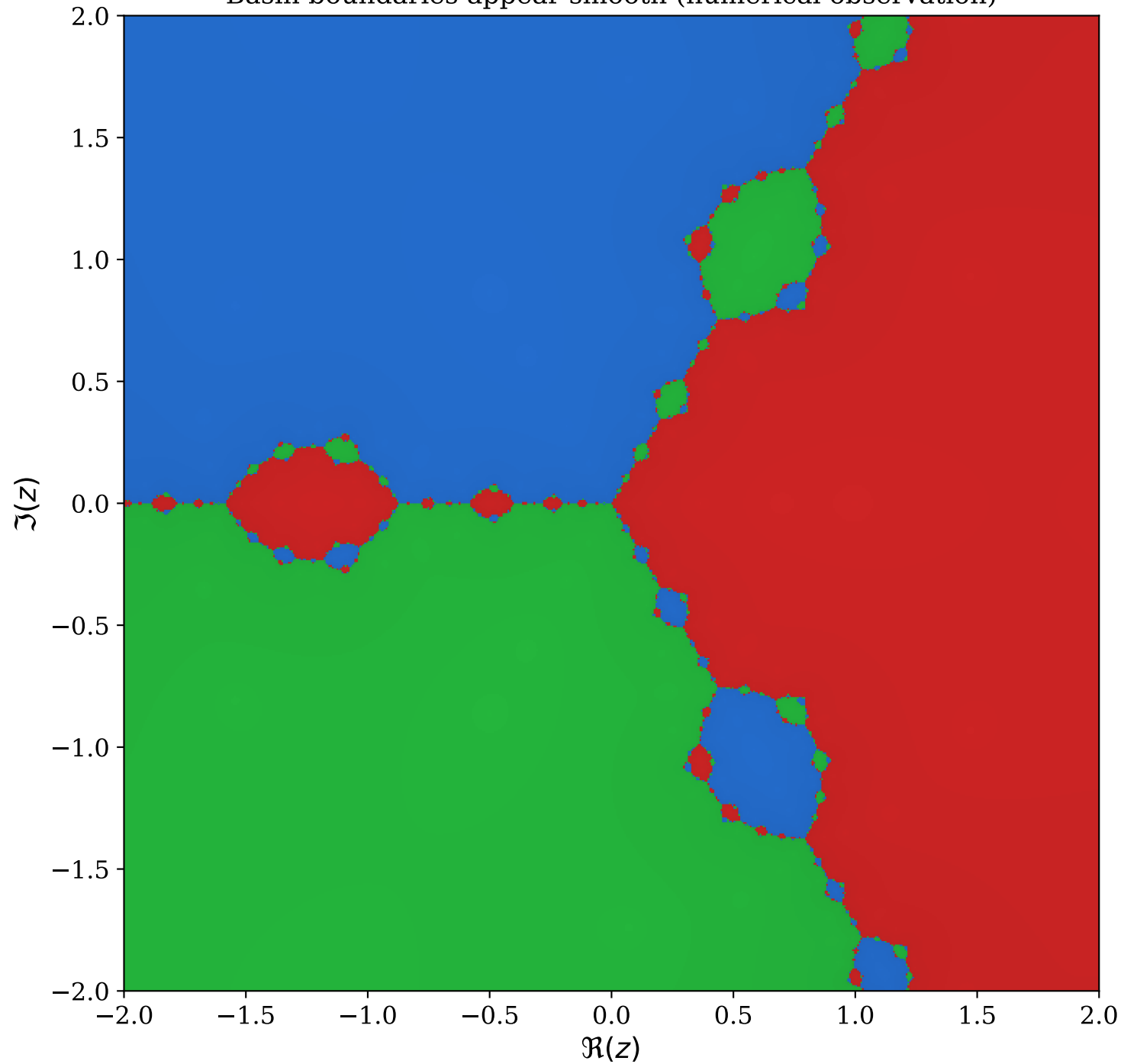
Pandrosion Iteration: z^3 - 1 Basin boundaries appear smooth (numerical observation)
