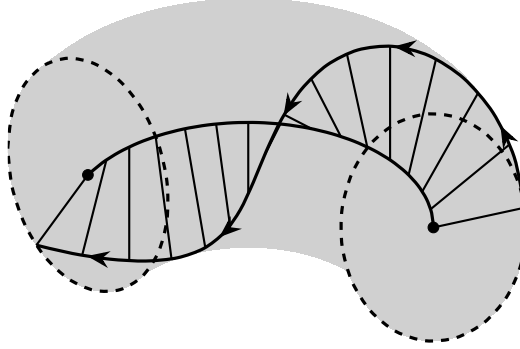
Figure 5.5: Magnetic field in a circular tokamak. The torus represents a surface \varrho = \text{const.} The ribbon is indeed a surface \beta = \text{const.} The intersection of the two is a curve of the coordinate \ell which follows a magnetic field-line.
