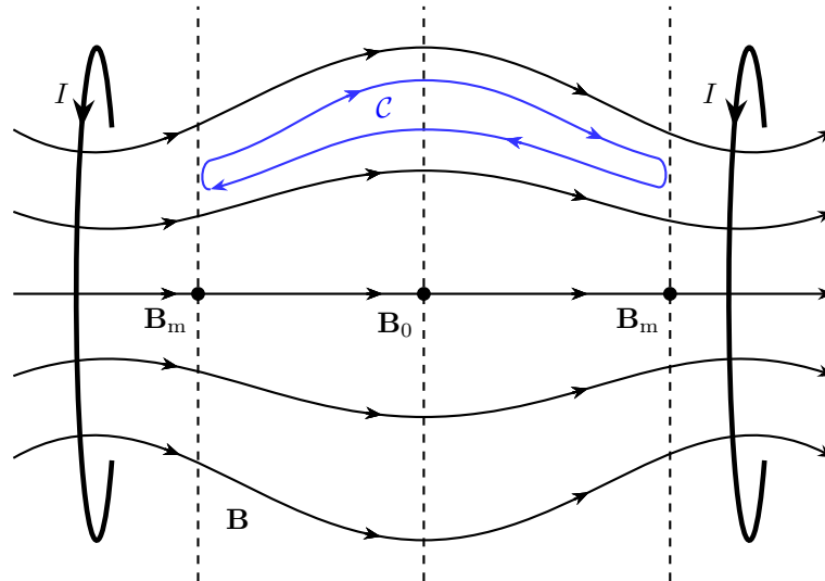
Figure 5.3: Magnetic mirrors and an illustrative trajectory of a confined particle.
