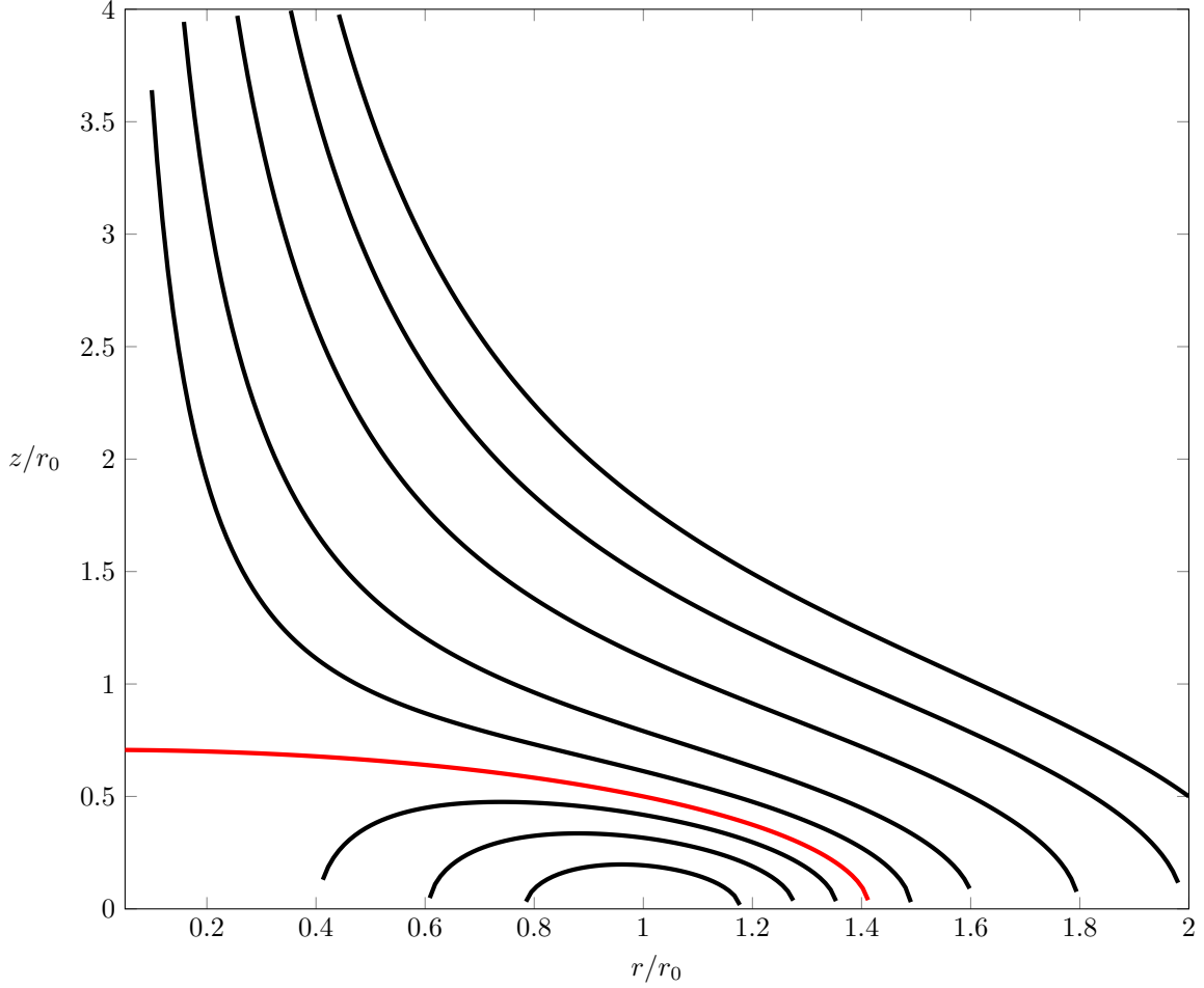
Figure 6.1: Magnetic surface contours according to Solovév's hypotheses, only in the upper half due to reflective symmetry about the horizontal plane. The red line is the separatrix , corresponding to zero poloidal disk flux and separating the open surfaces from closed ones.
