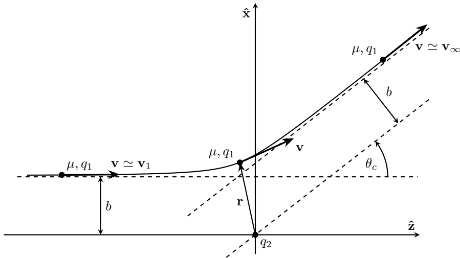
Figure 1.2: Illustration of the binary Coulomb collision problem.
