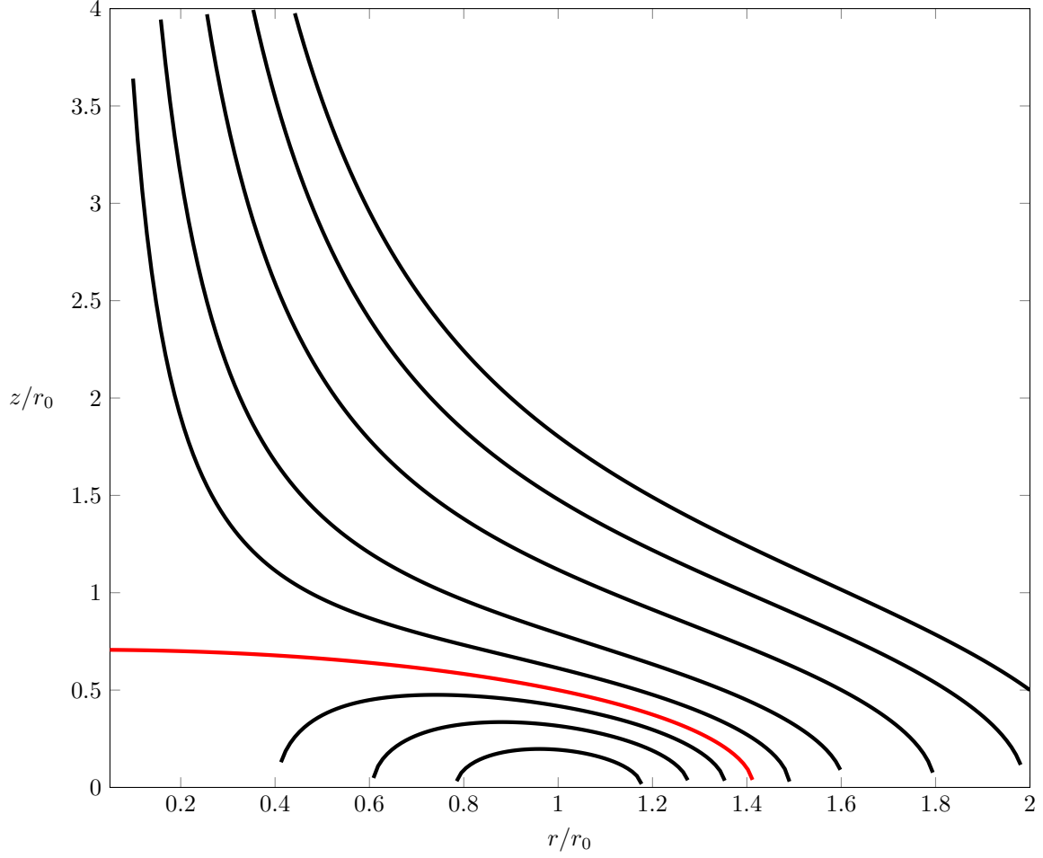
Figure 6.1: Magnetic surface contours according to Solov'ev's hypotheses, only in the upper half due to reflective symmetry about the horizontal plane. The red line is the separatrix , corresponding to zero poloidal disk flux and separating the open surfaces from closed ones.
