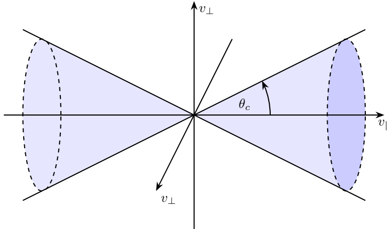
Figure 2.1: Loss cone
