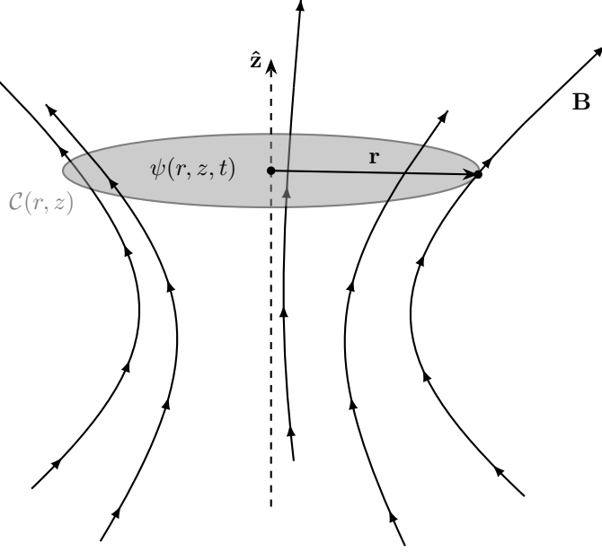
Figure 2.2: Poloidal \mathbf{B} . The flux through \mathcal{C}(r, z) is \psi(r, z, t) .
