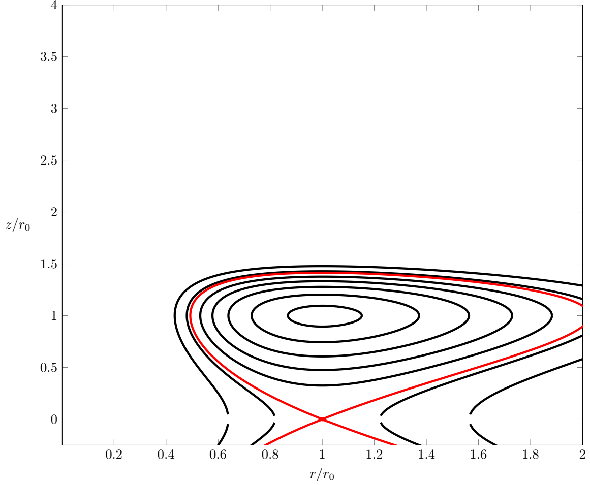
Figure 8.1: Magnetic surface contours topologically equivalent to those in tokamaks. The separatrix corresponding to zero magnetic flux is traced in red.
