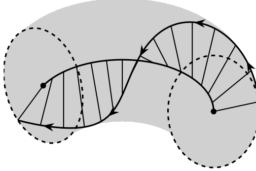
Figure 5.2: Magnetic field in a circular tokamak. The torus represents a surface \varrho = \text{const.} The ribbon is indeed a surface \beta = \text{const.} The intersection of the two is a curve of the coordinate \ell which follows a magnetic field-line.
