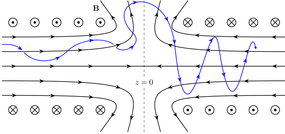
Figure 2.3: Lines of \mathbf{B} and trajectory of a particle crossing the cusp in blue.
