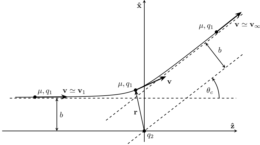
Figure 1.2: Illustration of the binary Coulomb collision problem.
