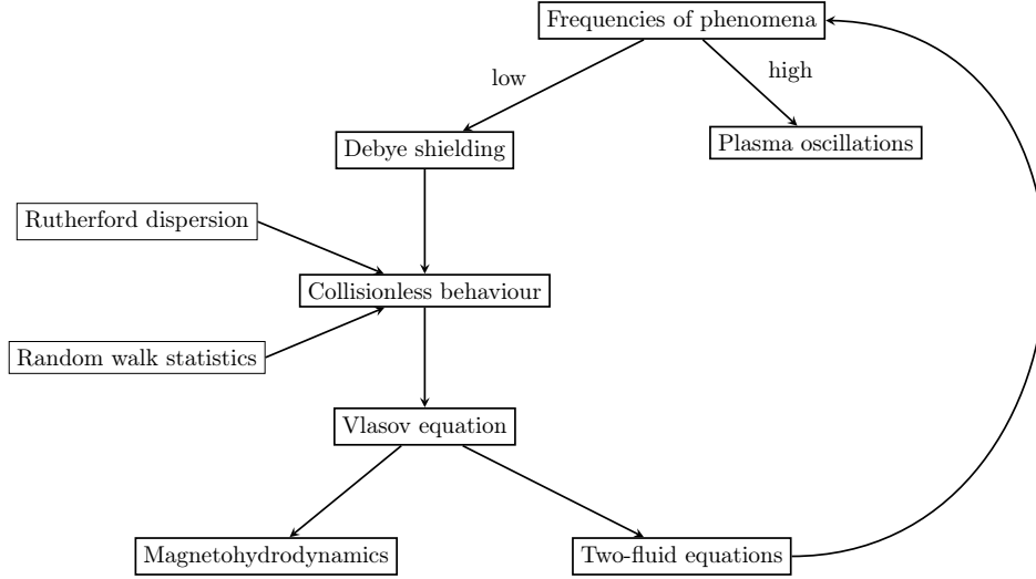
Figure 1.1: Hierarchy of plasma models
