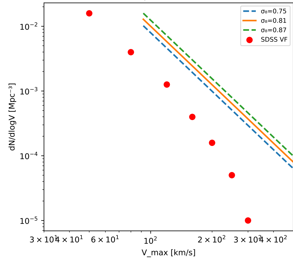
(a) Velocity Function: \sigma_8 + RAR
