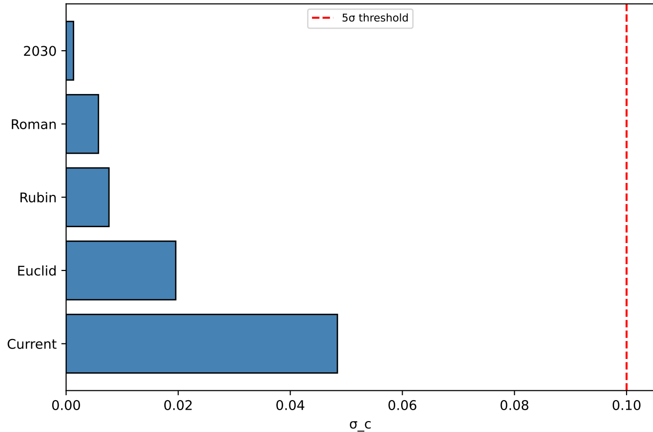
(b) Forecast ( \sigma_{\text{sys}} = 0.05 dex, \sigma_{c,\text{current}} = 0.048 )
