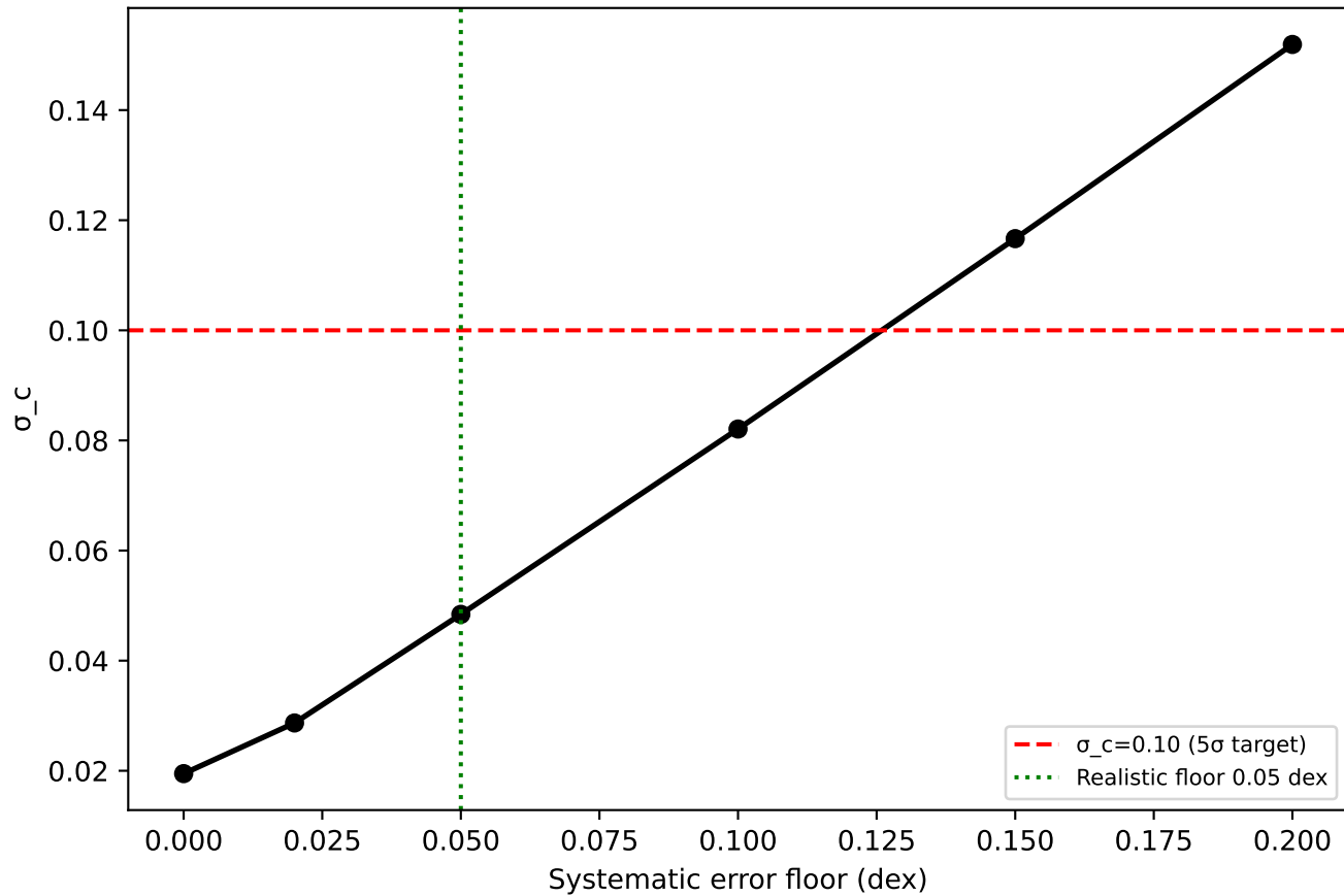
(a) \sigma_c vs Systematic Floor (Monte Carlo)
