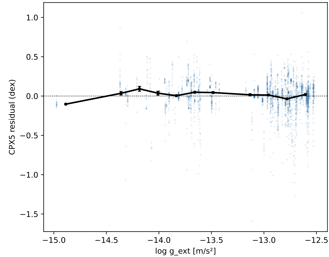
Per-galaxy: \rho=-0.1044 ( p=1.69\text{e-}01 )
