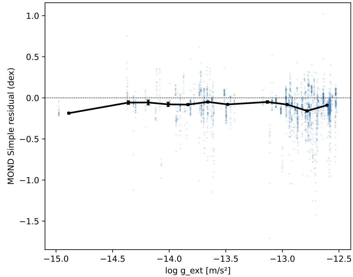
Per-galaxy: \rho=-0.1057 ( p=1.64\text{e-}01 )
