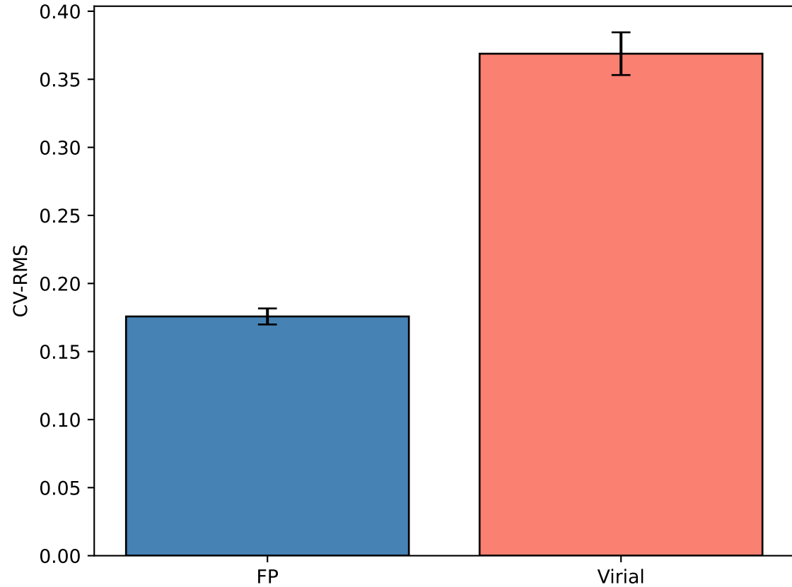
10-Fold CV
