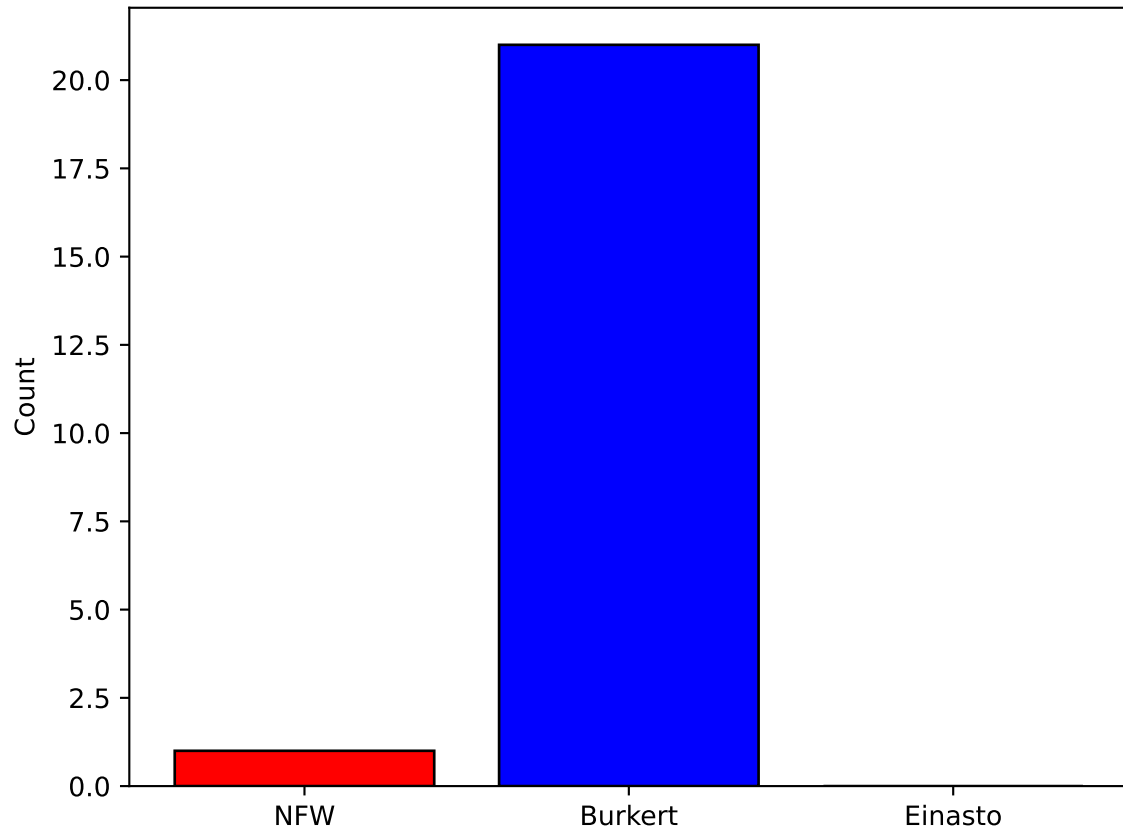
Best Model (22 galaxies, \chi^2_{\text{red}} < 20 )
