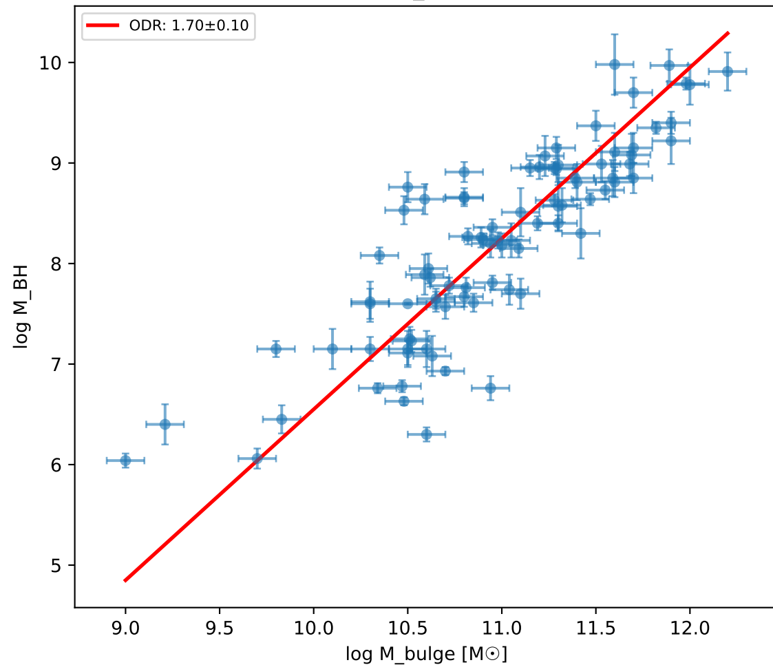
M-M_bulge
