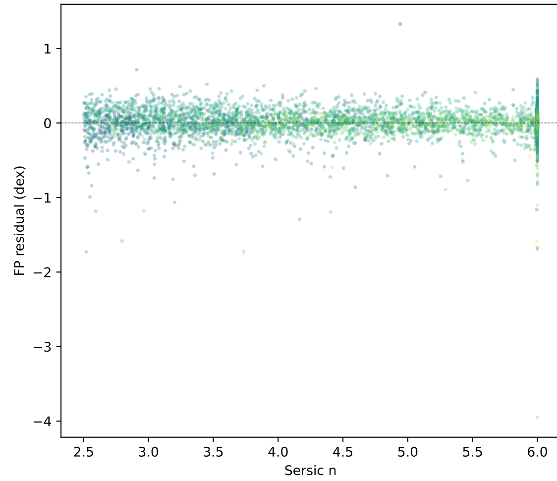
(c) Residual vs Sersic n ( \rho=-0.005 )
