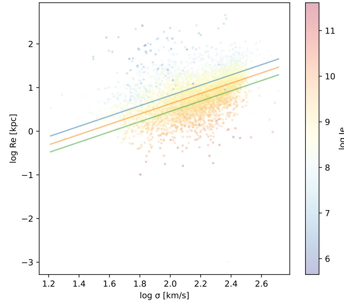
(a) Fundamental Plane (5429 galaxies, RMS=0.176)
