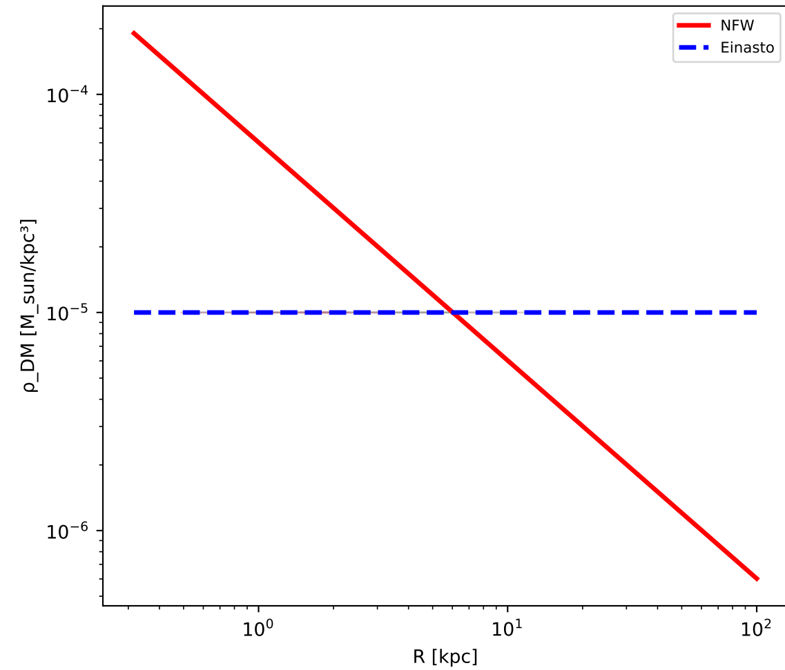
(a) DM Density Profiles
