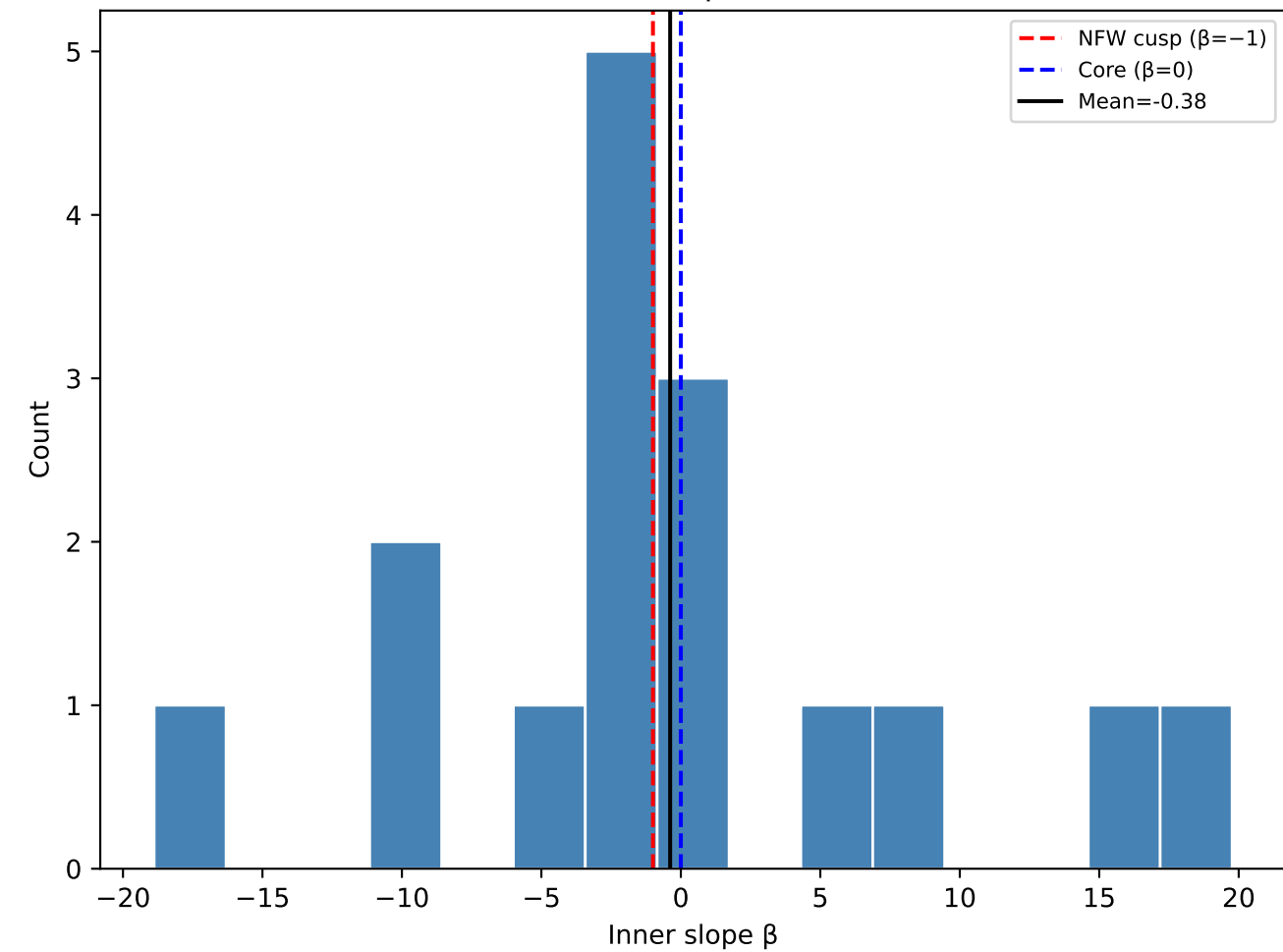
(a) Inner DM Slope Distribution
