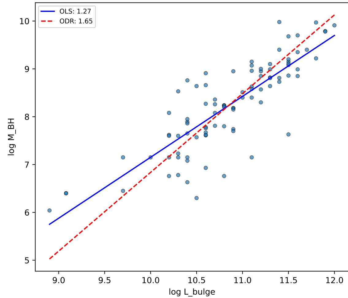
M-L: RMS=0.511
