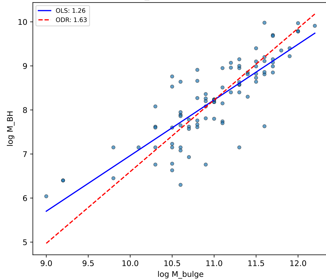
M-M_bulge: RMS=0.510
